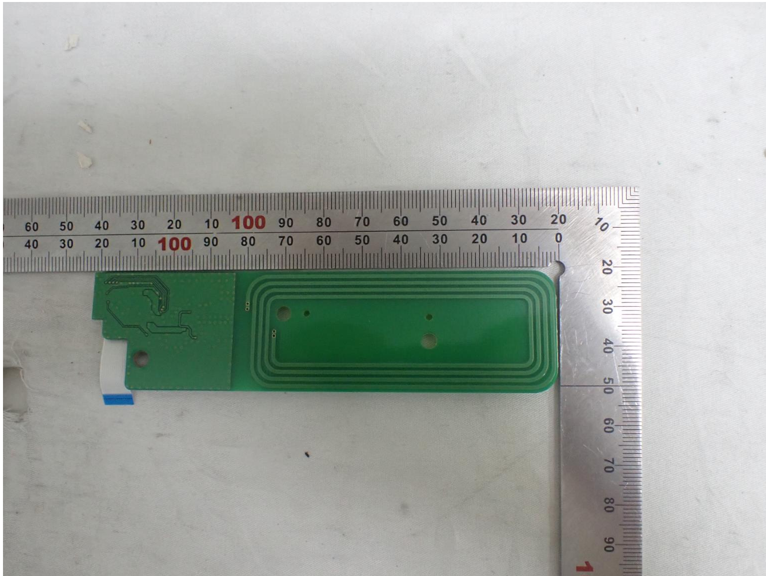
RF ANT BOARD rear
