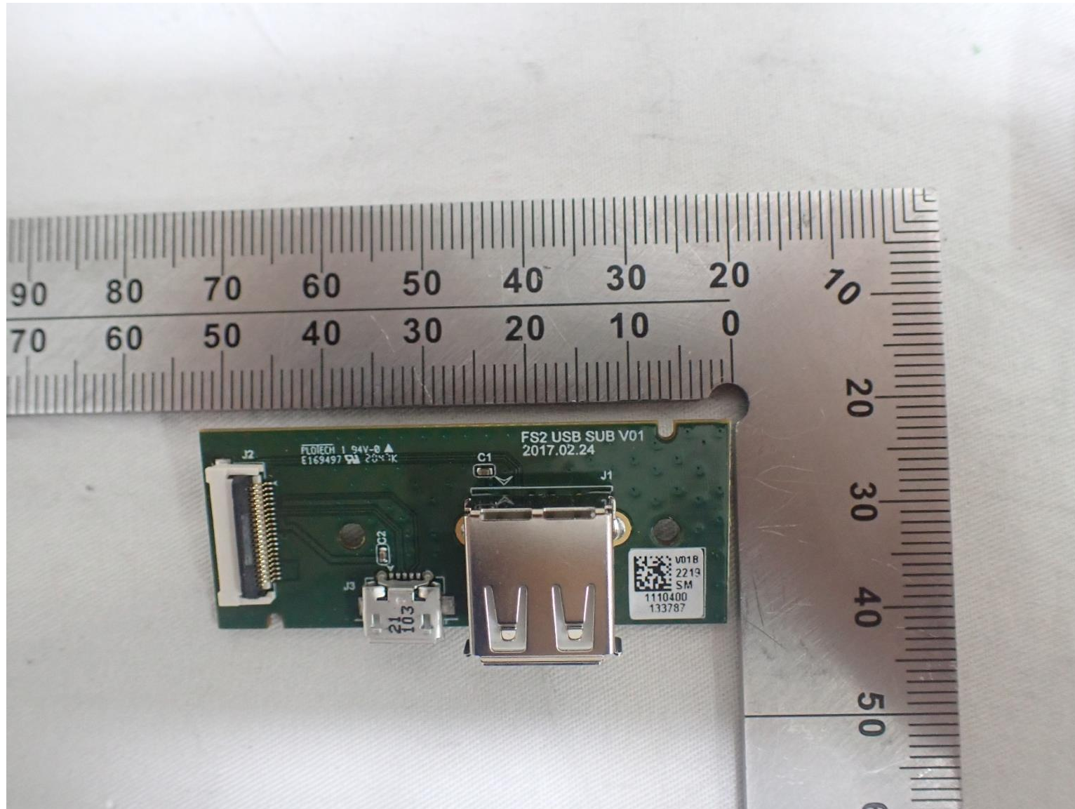
USB SUB front
