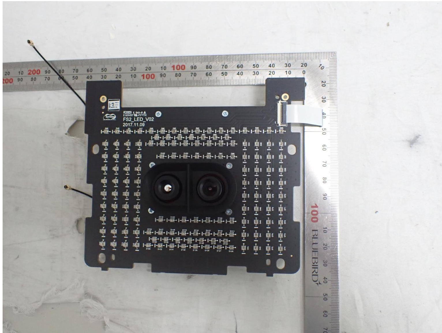
LED BOARD front
