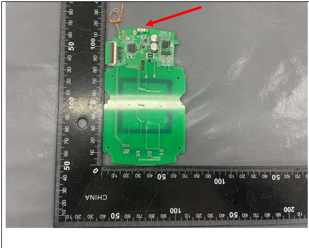
Chip Antenna (Bluetooth LE)
