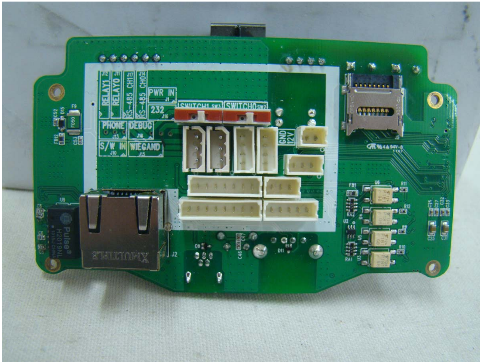
IO BOARD FRONT
