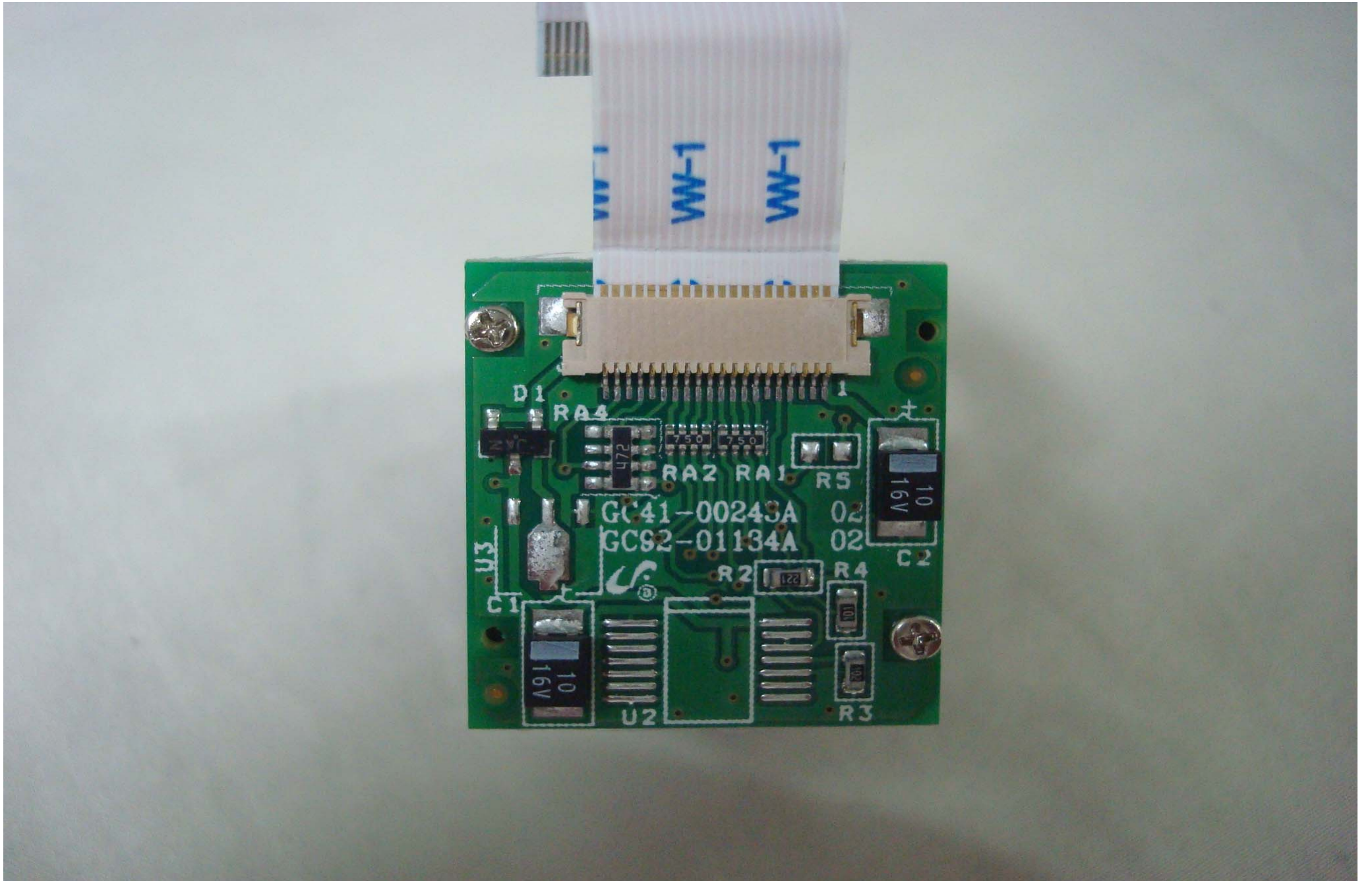
FINGER SCAN BOARD 전면
