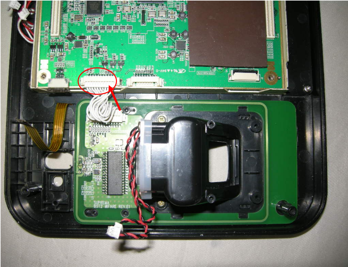
RF antenna location(attached Card logo part of the front side)
