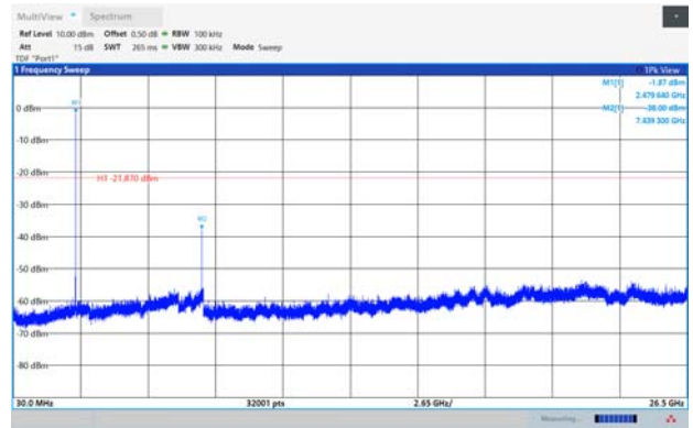
Conducted spurious / 2 480 MHz
