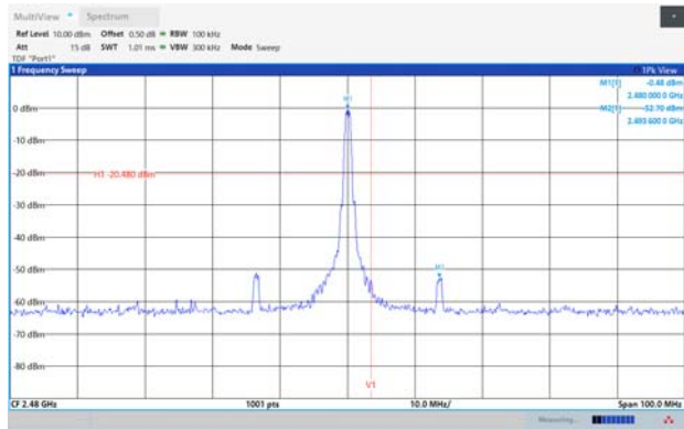
Conducted band-edge / 2 480 MHz
