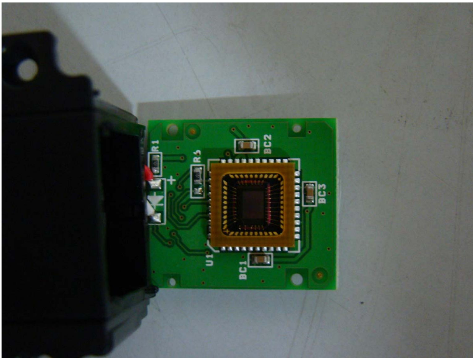
FINGER SCANNER MODULE BOARD FRONT
