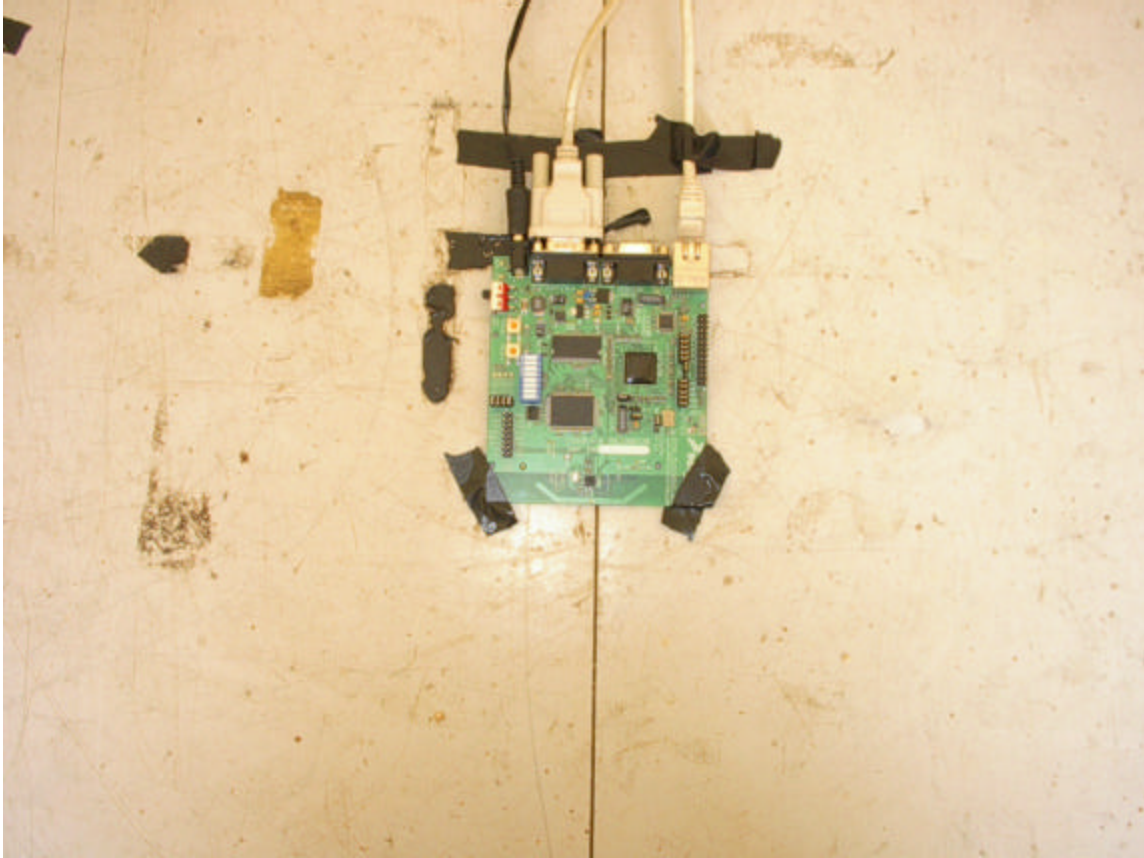
Emissions Test Setup Top View
