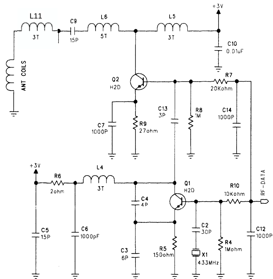
TRNSMIE BOARD.SCH
