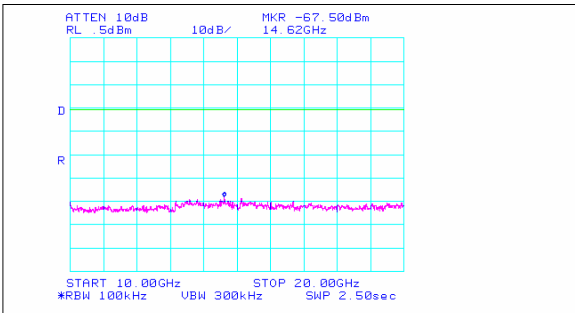
Plot 18. Spurious Conducted Emission – Channel 0 – 10 GHz to 20 GHz*
