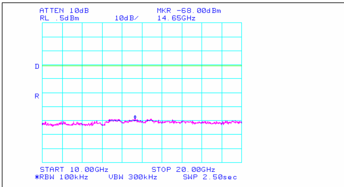
Plot 26. Spurious Conducted Emission – Channel 7 – 10 GHz to 20 GHz*
