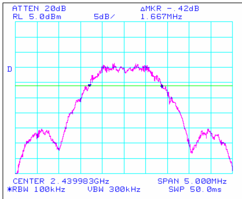
Plot 2. Occupied Bandwidth – Channel 7
