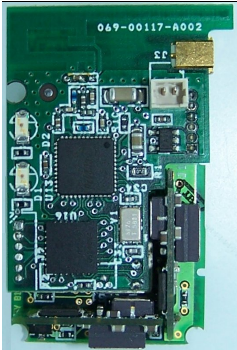
Photograph 6. Sample Used for Conducted Testing
