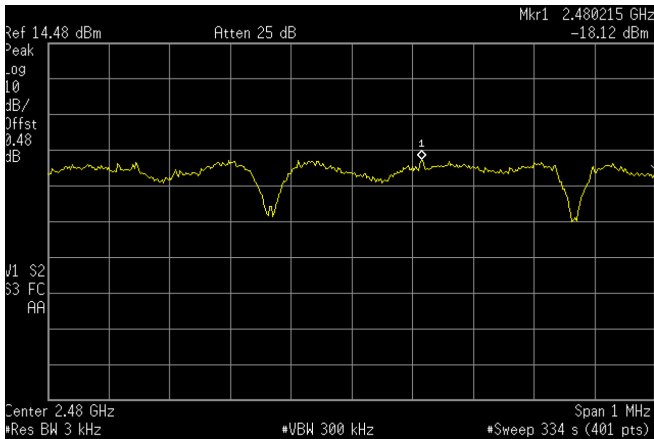
Plot 11. Spectral Power Density – Channel 15
