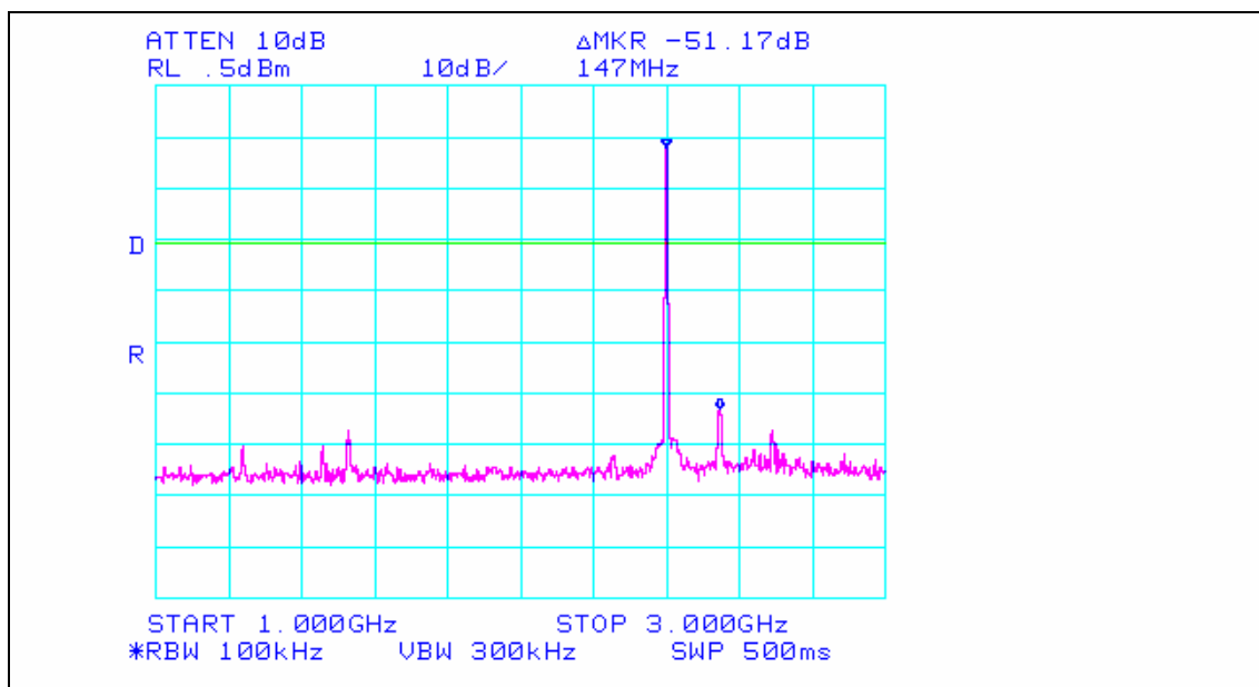
Plot 15. Spurious Conducted Emission – Channel 0 – 1 GHz to 3 GHz
