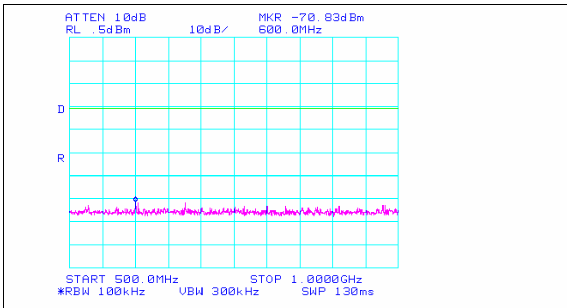
Plot 30. Spurious Conducted Emission – Channel 15 – 500 MHz to 1 GHz*
