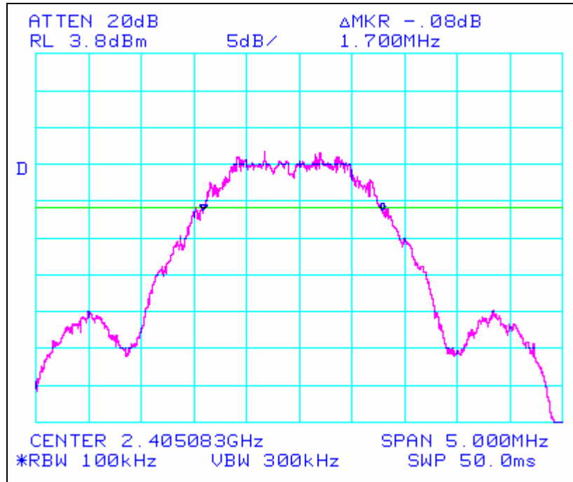
Plot 1. Occupied Bandwidth – Channel 0
