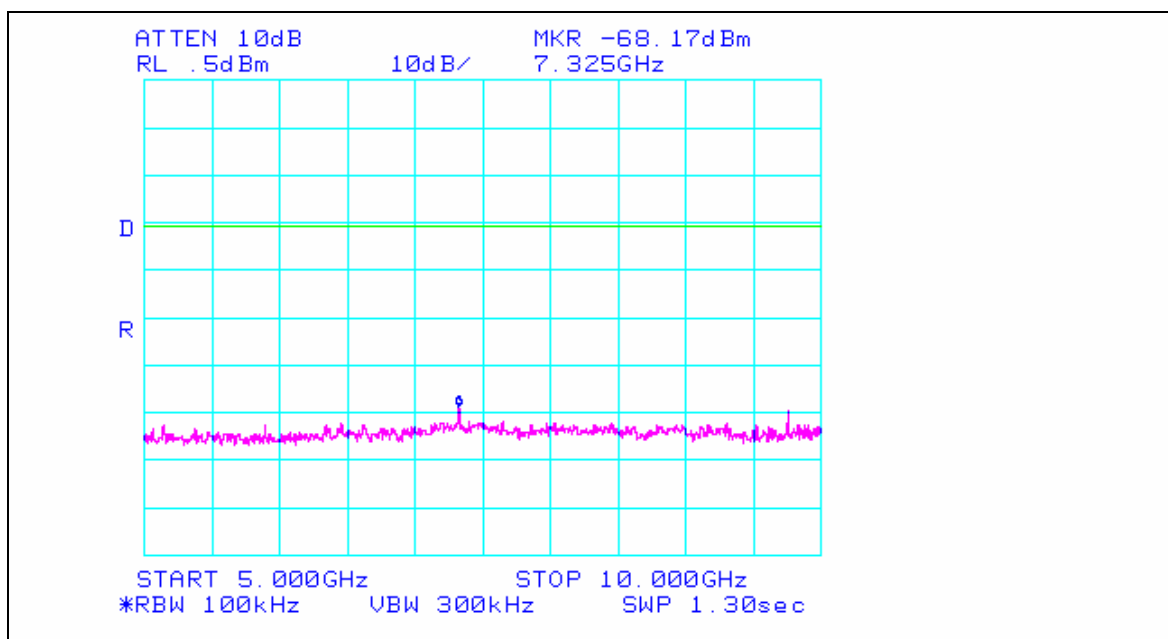
Plot 25. Spurious Conducted Emission – Channel 7 – 5 GHz to 10 GHz*
