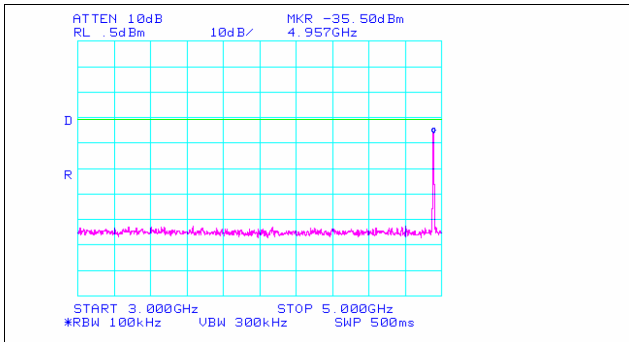
Plot 32. Spurious Conducted Emission – Channel 15 – 3 GHz to 5 GHz*
