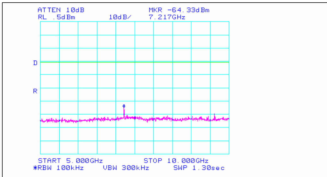
Plot 17. Spurious Conducted Emission – Channel 0 – 5 GHz to 10 GHz*
