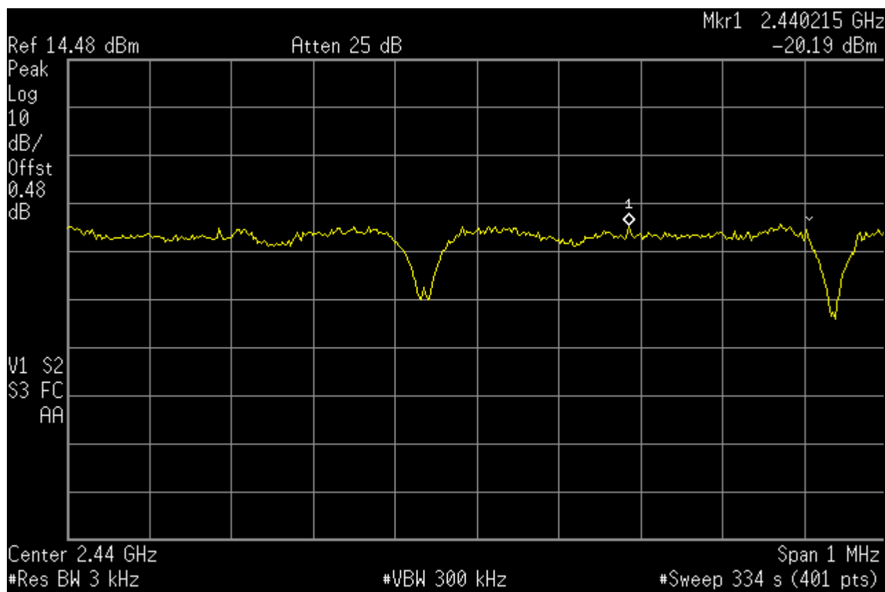
Plot 10. Spectral Power Density – Channel 7
