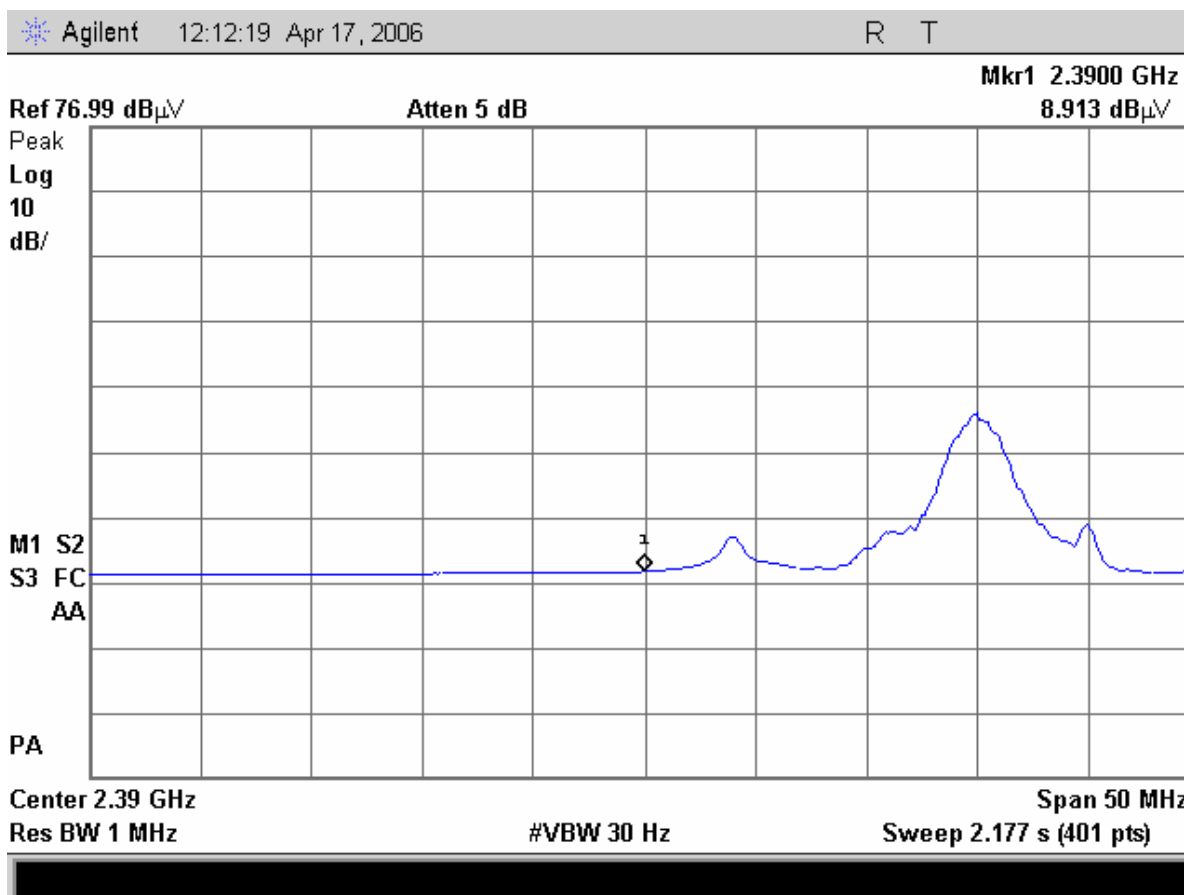
Plot 7. Band Edge Emissions Channel 0
