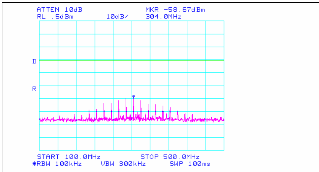
Plot 21. Spurious Conducted Emission – Channel 7 – 100 MHz to 500 MHz*
