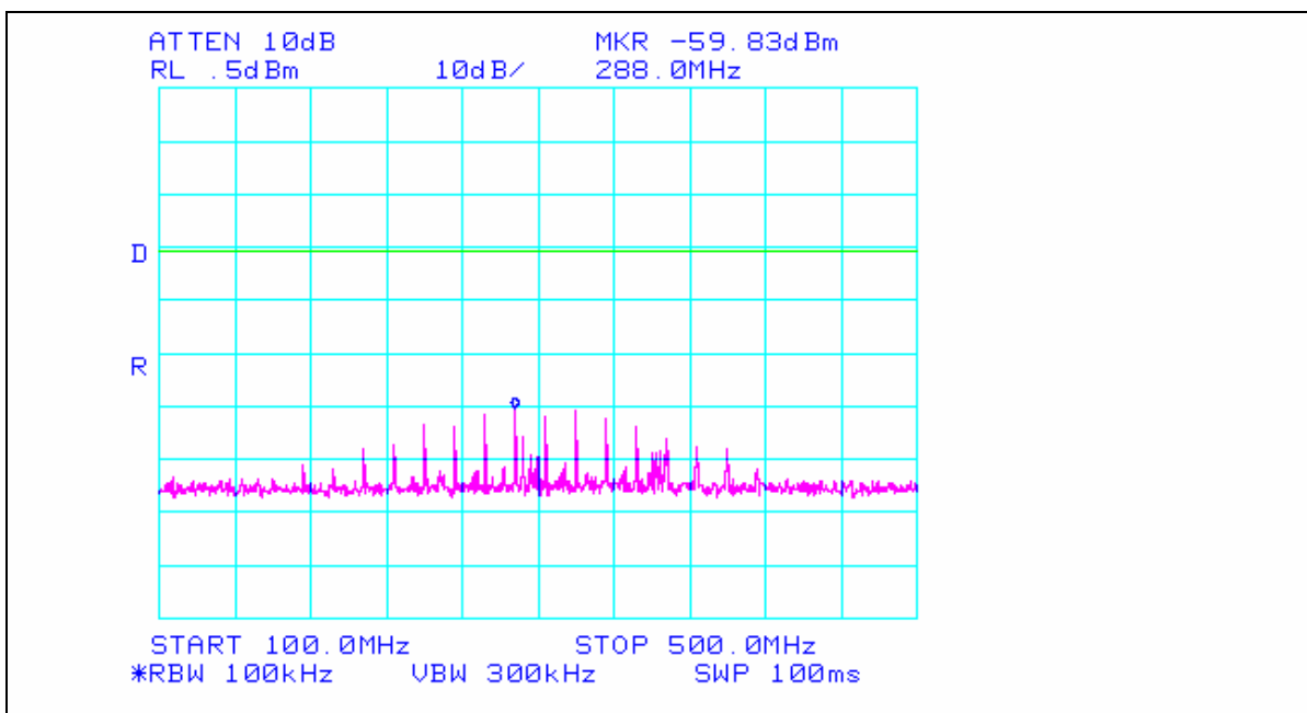
Plot 13. Spurious Conducted Emission – Channel 0 – 100 MHz to 500 MHz*
