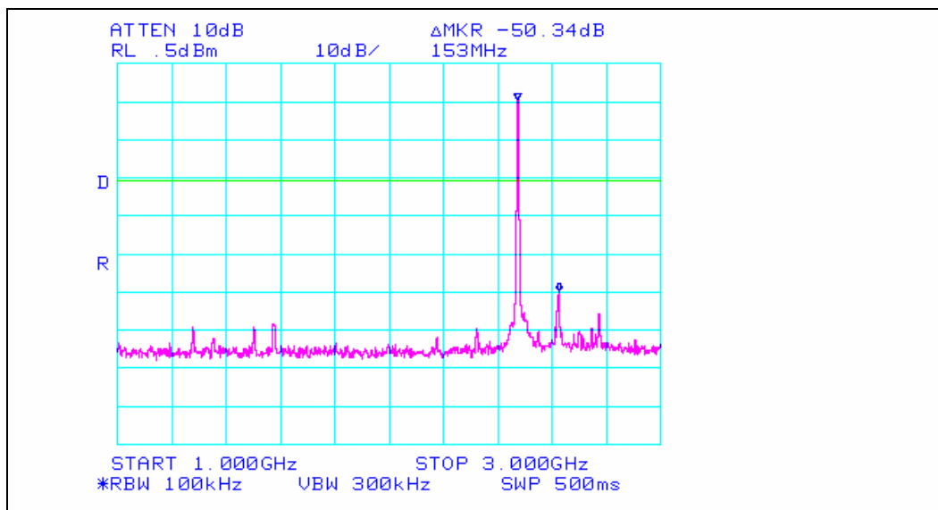
Plot 31. Spurious Conducted Emission – Channel 15 – 1 GHz to 3 GHz*
