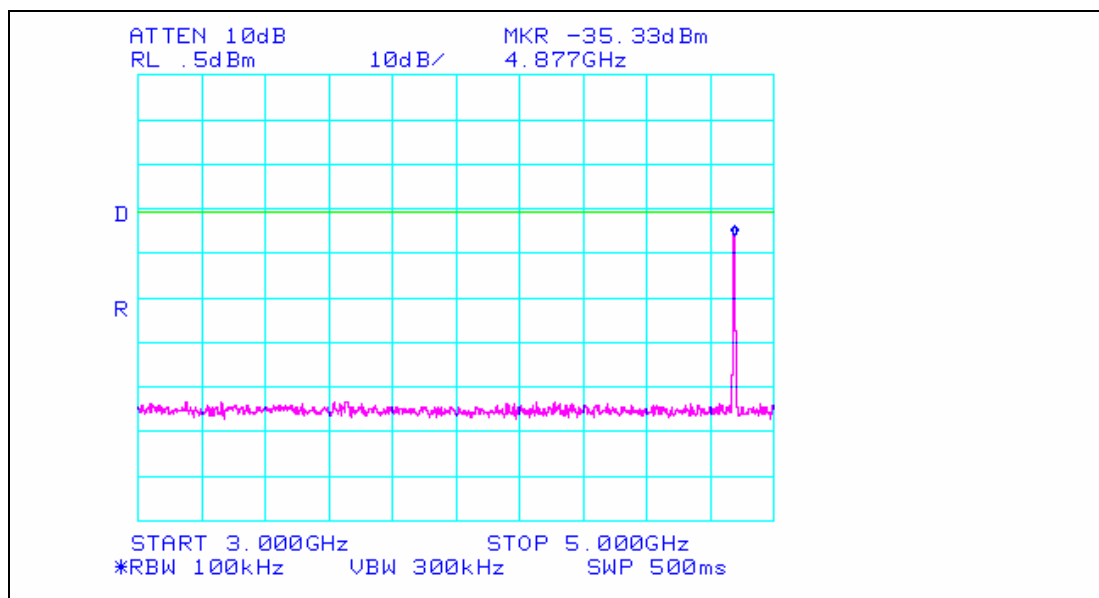
Plot 24. Spurious Conducted Emission – Channel 7 – 3 GHz to 5 GHz*
