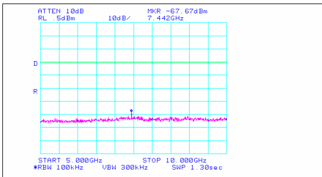
Plot 33. Spurious Conducted Emission – Channel 15 – 5 GHz to 10 GHz*
