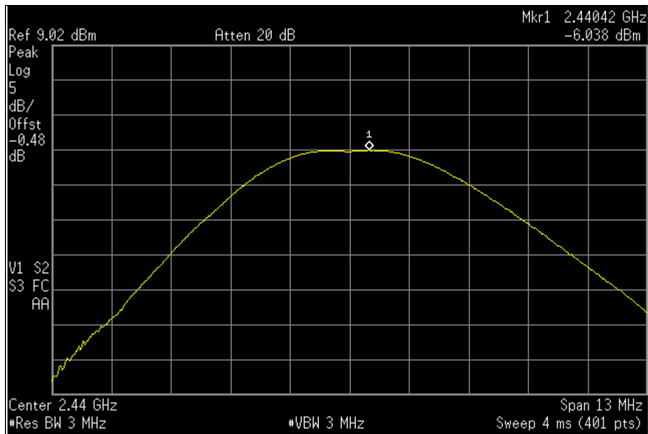
Plot 5. Output Power – Channel 7
