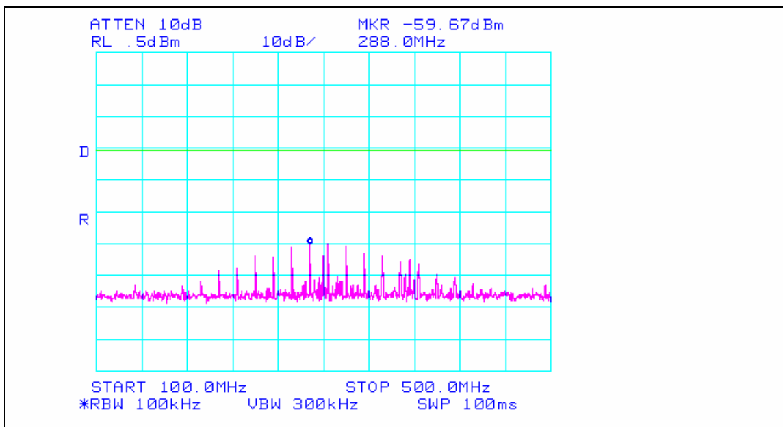
Plot 29. Spurious Conducted Emission – Channel 15 – 100 MHz to 500 MHz*
