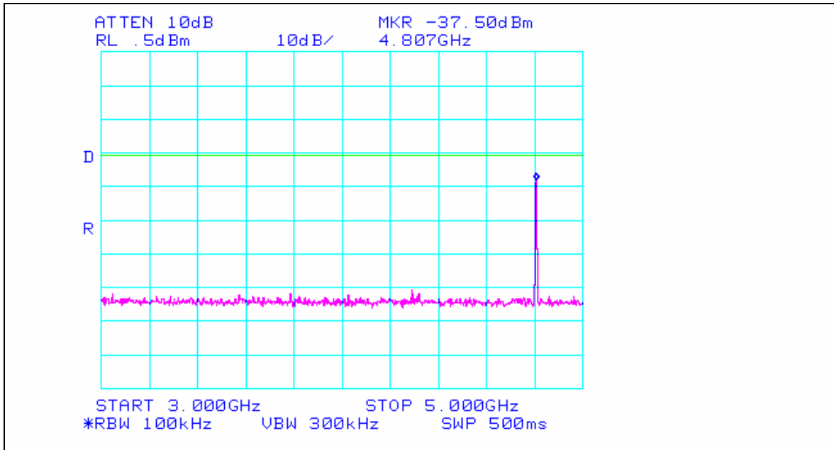
Plot 16. Spurious Conducted Emission – Channel 0 – 3 GHz to 5 GHz*
