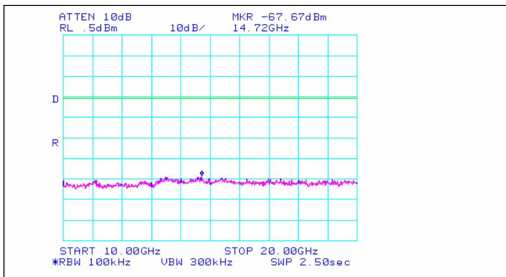
Plot 34. Spurious Conducted Emission – Channel 15 – 10 GHz to 20 GHz*
