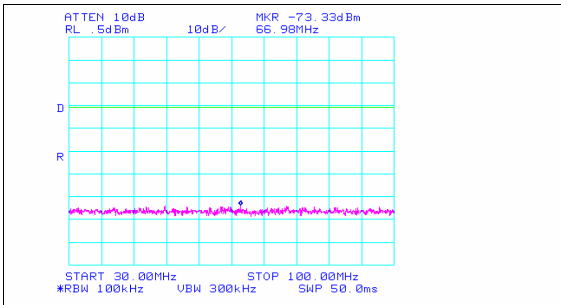
Plot 28. Spurious Conducted Emission – Channel 15 – 30 MHz to 100 MHz*
