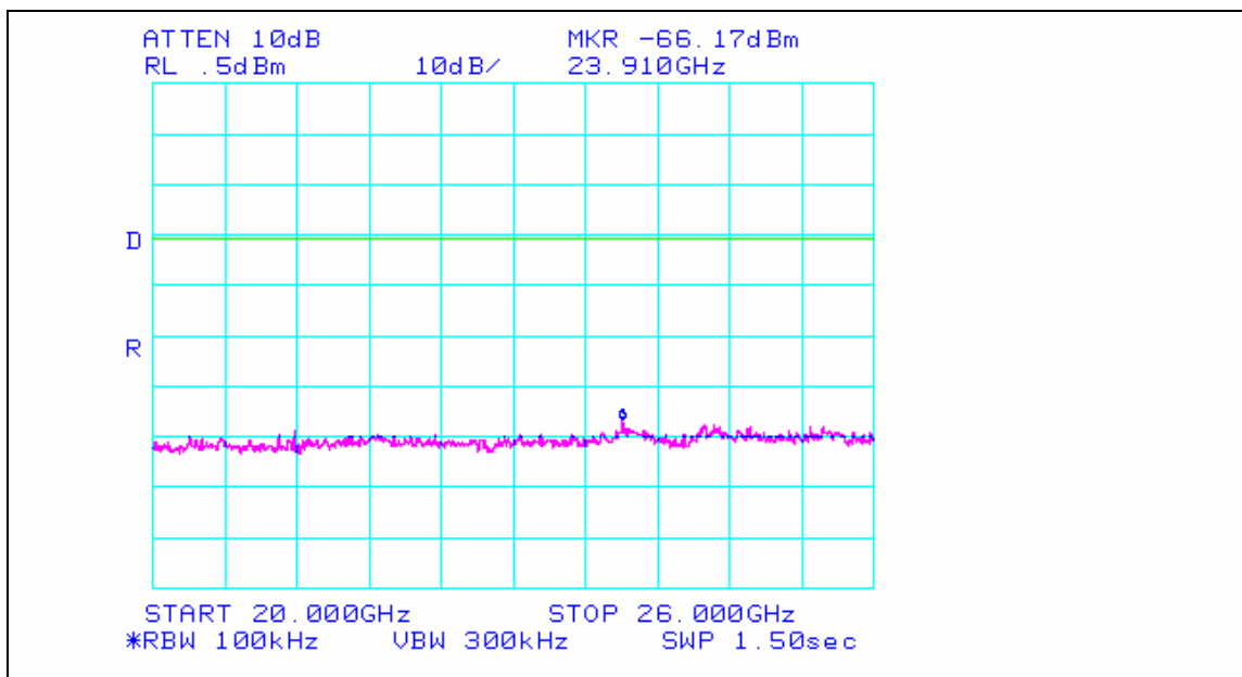
Plot 27. Spurious Conducted Emission – Channel 7 – 20 GHz to 26 GHz*
