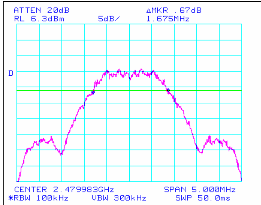
Plot 3. Occupied Bandwidth – Channel 15
