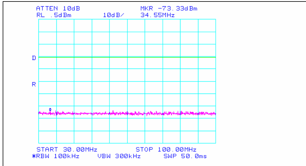
Plot 20. Spurious Conducted Emission – Channel 7 – 30 MHz to 100 MHz*
