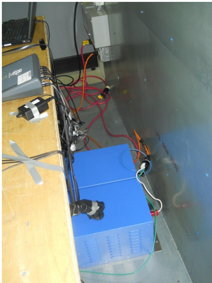
AC mains conducted emissions
