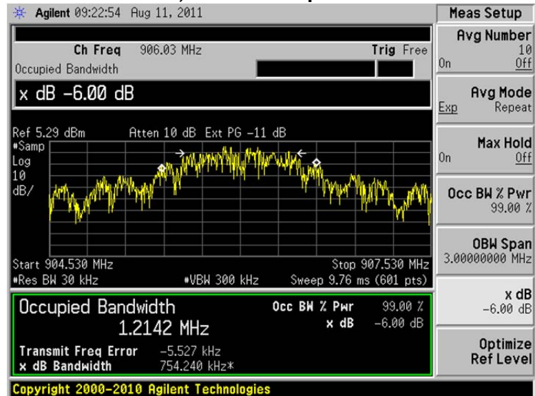
Channel 1, -6 dBc Occupied Bandwidth
