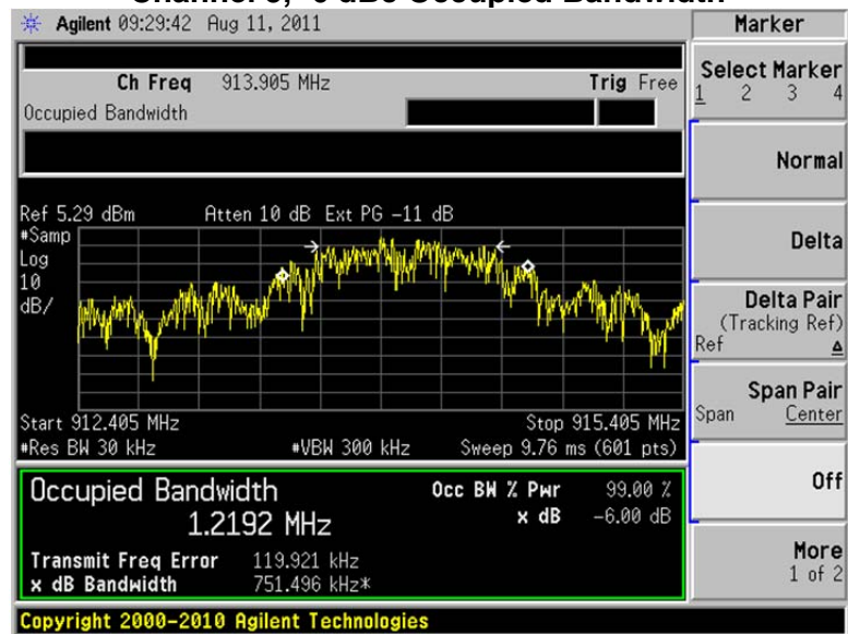
Channel 5, -6 dBc Occupied Bandwidth
