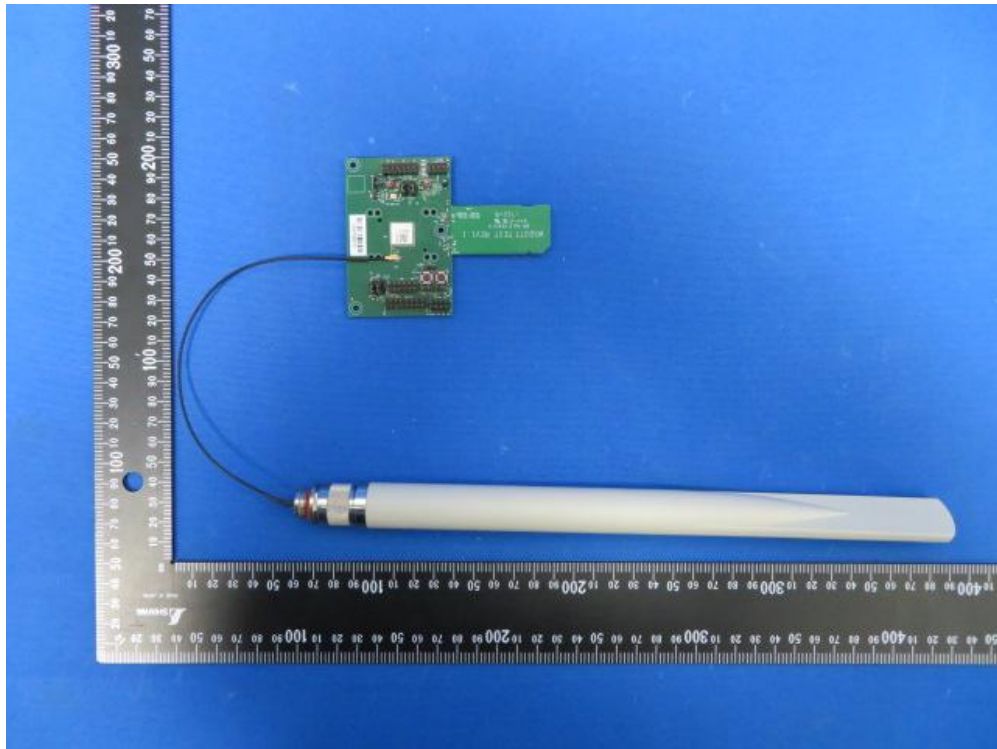
(4) EUT Photo (Detail antenna matching lay on the test jig)
