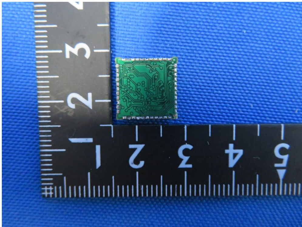
(2) EUT Photo (Module)
