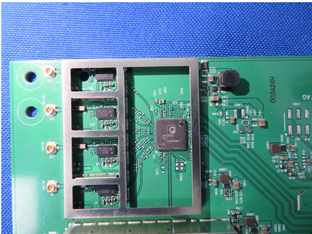
(14) EUT Photo (4x4 Indoor 11ax AP with Internal Antenna)
