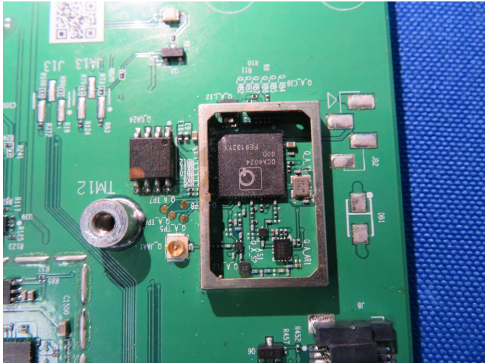
(28) EUT Photo (4x4 Indoor 11ax AP with External SMA Connector)
