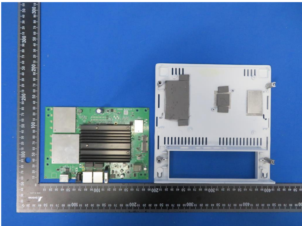
(20) EUT Photo (4x4 Indoor 11ax AP with External SMA Connector)
