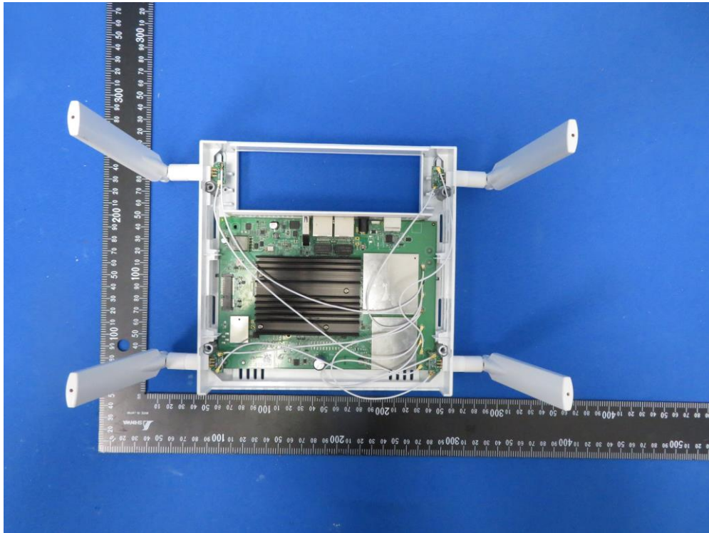
(18) EUT Photo (4x4 Indoor 11ax AP with External SMA Connector)
