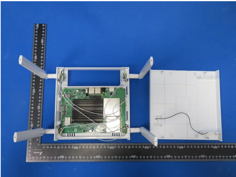
(16) EUT Photo (4x4 Indoor 11ax AP with External SMA Connector)
