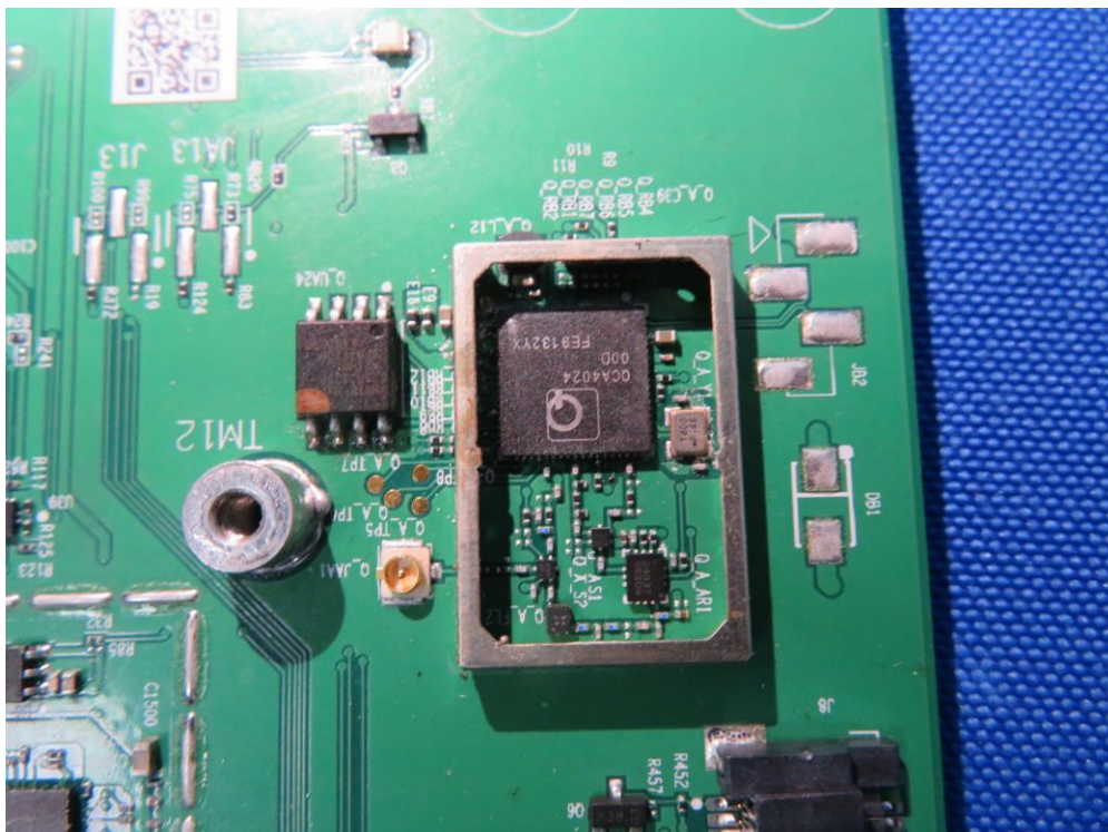
(12) EUT Photo (4x4 Indoor 11ax AP with Internal Antenna)
