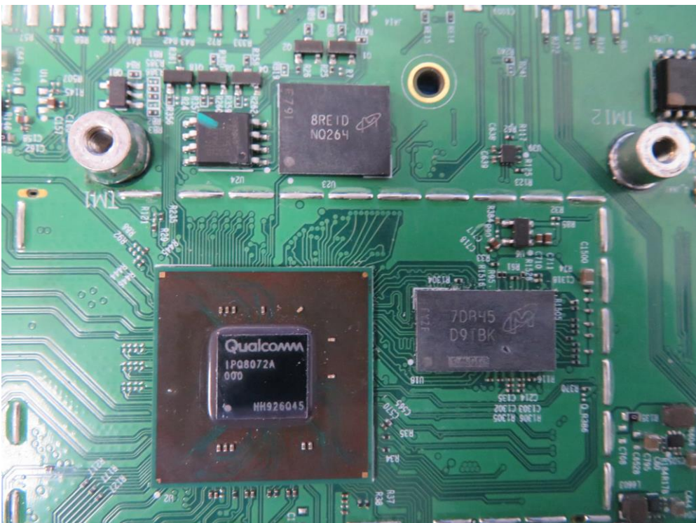
(26) EUT Photo (4x4 Indoor 11ax AP with External SMA Connector)
