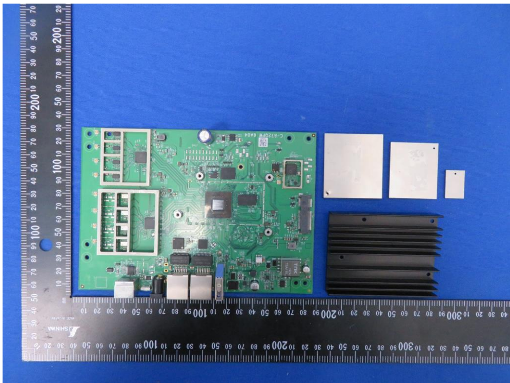
(8) EUT Photo (4x4 Indoor 11ax AP with Internal Antenna)
