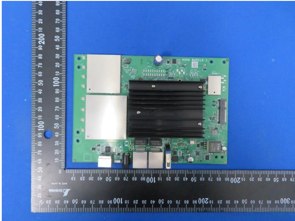
(22) EUT Photo (4x4 Indoor 11ax AP with External SMA Connector)
