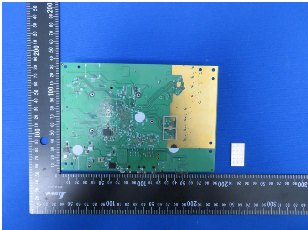
(24) EUT Photo (4x4 Indoor 11ax AP with External SMA Connector)
