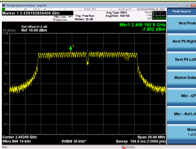
Channel 11 (2462MHz)
