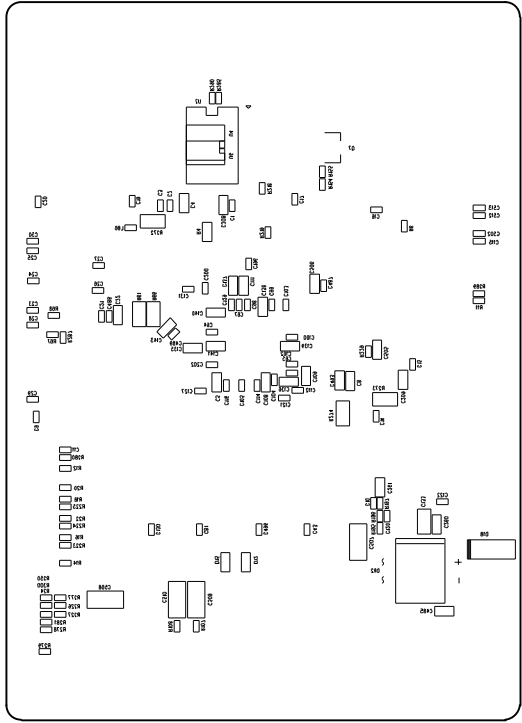
Silkscreen bottom
