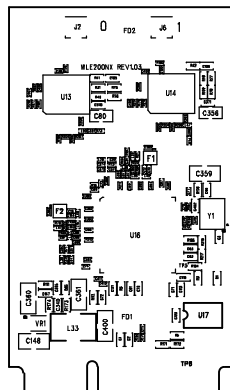
Silkscreen top
