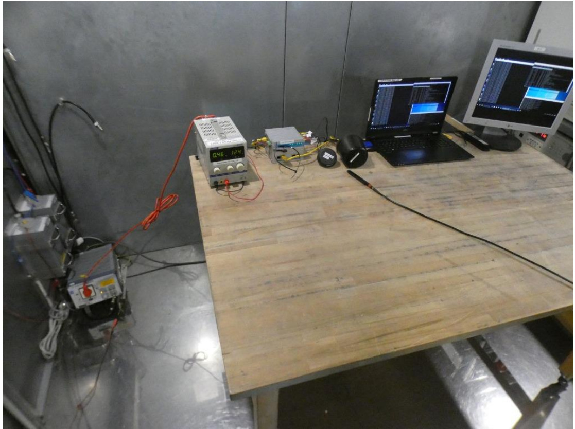
Photo 6: Test setup for conducted measurements FCC15b.
