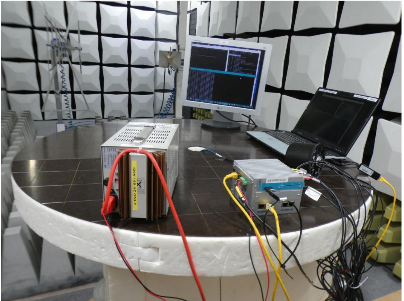
Photo 4: Test setup for radiated measurements FCC15b, 18 GHz – 26 GHz
