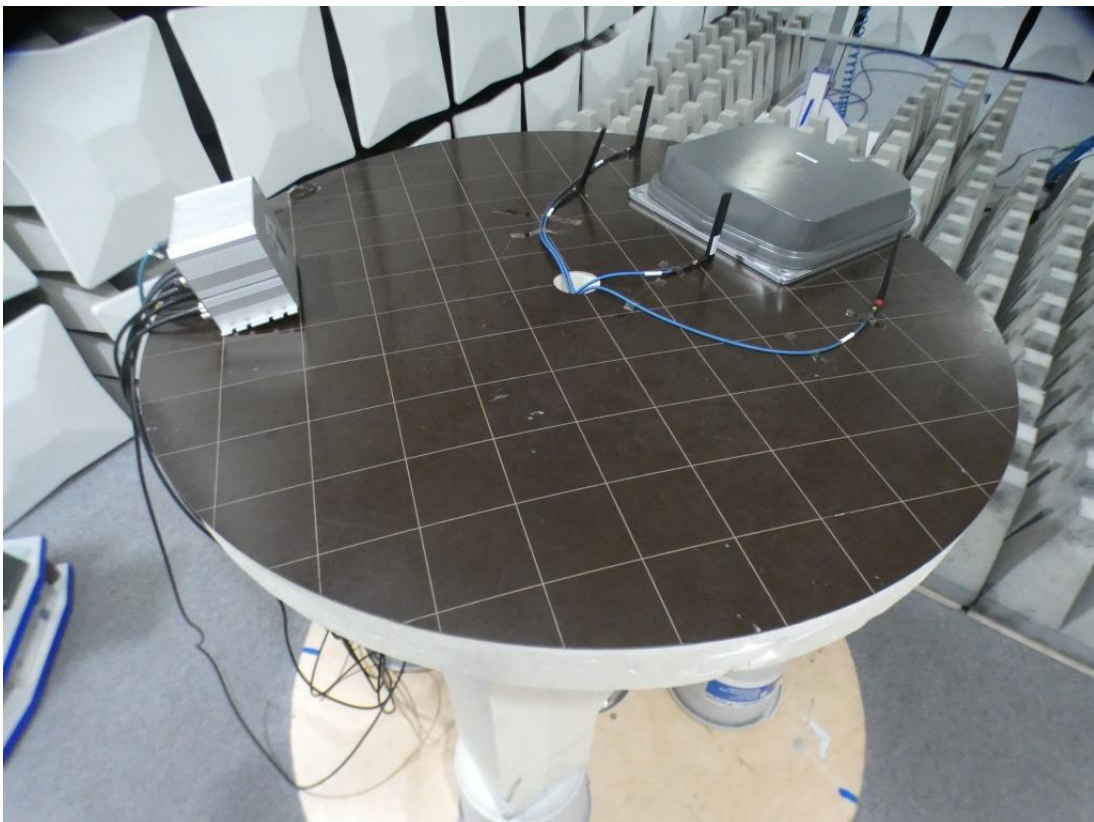
Photo 2: Test setup S01_AA01 for radiated emissions measurements - Detailed view
