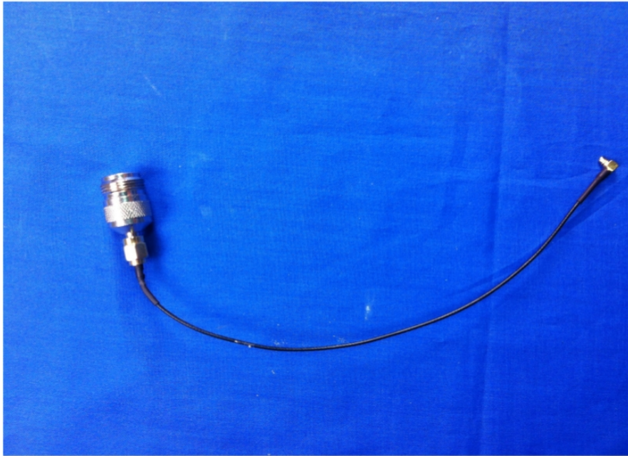
9) EUT Photo (connector for 7dBi antenna)
