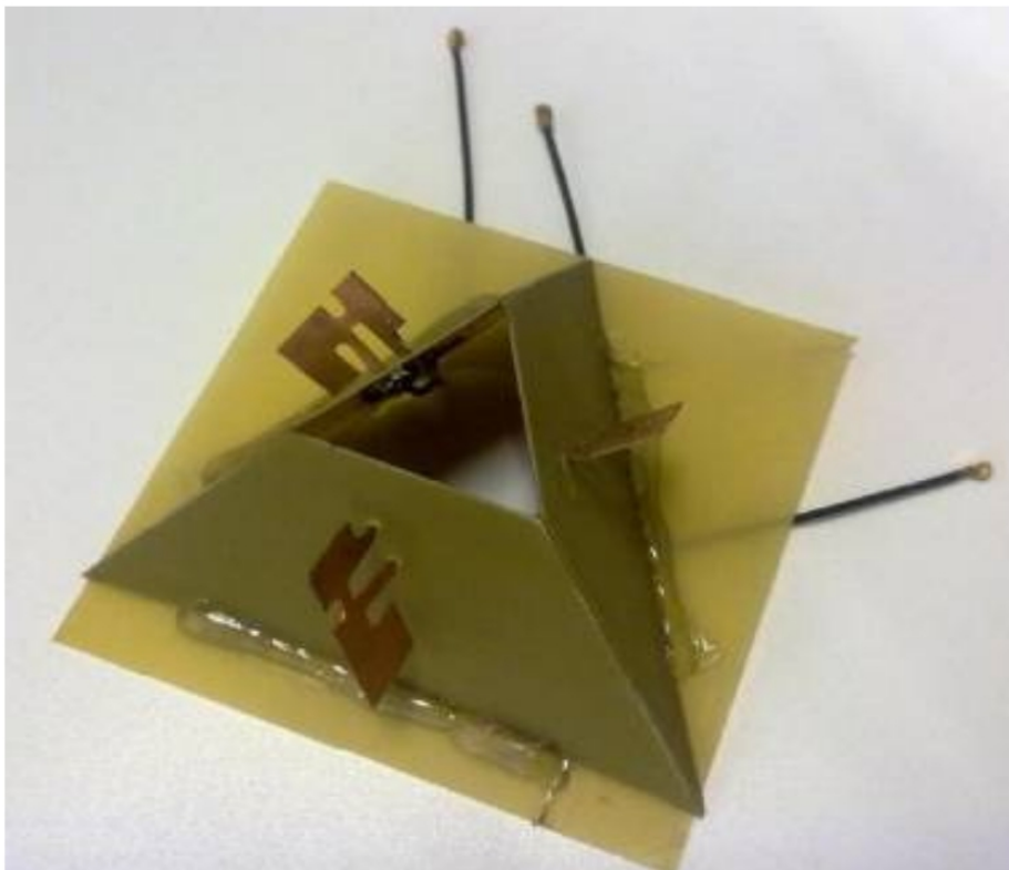
10) EUT Photo (5dBi antenna fixed with cable)
