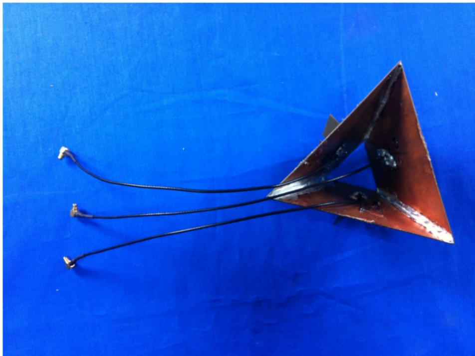
11) EUT Photo (5dBi antenna fixed with cable)
