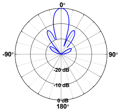
H-Pol Elevation (Port 2 – V)
