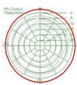
Gain: 3.12dBi
