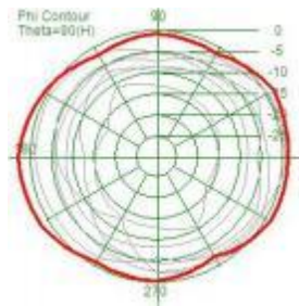
Gain: 2.89dBi
