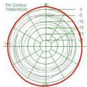
Gain: 3.34dBi
