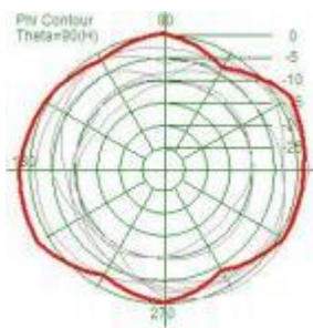
Gain: 2.98dBi
