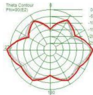
Efficiency:55.25%
