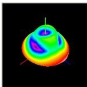
2.45GHz
