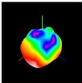
5.825GHz
