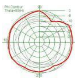
Gain: 3.33dBi
