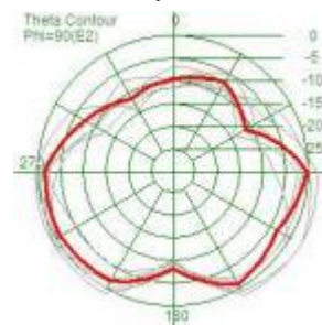
Efficiency: 67.88%
