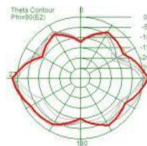
Efficiency:64.32%
