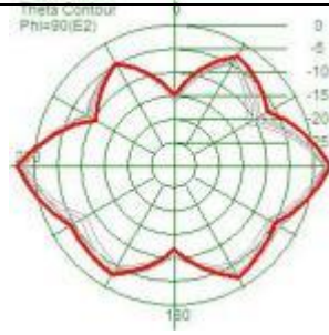
Efficiency: 67.12%
