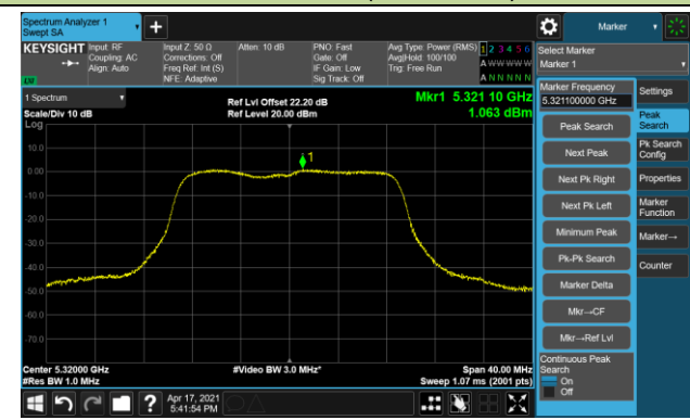
Channel 64 (5320MHz)
