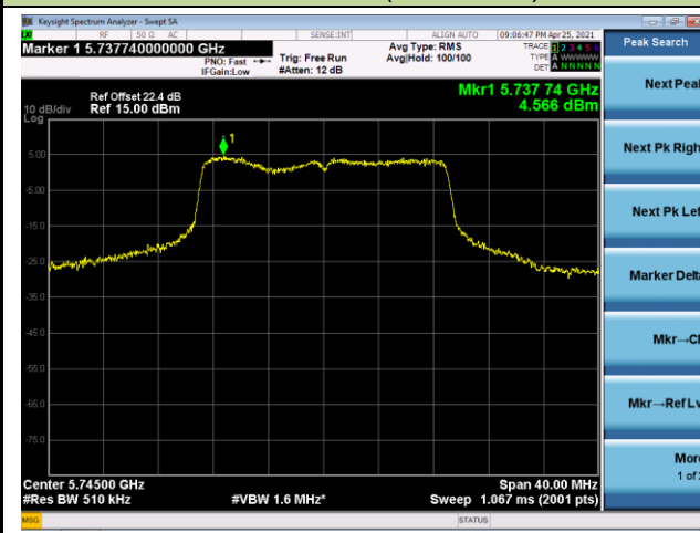
Channel 149 (5745MHz)
