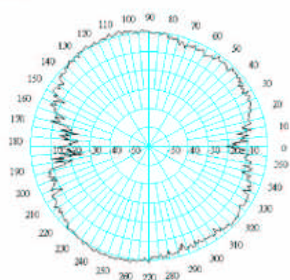
5.15-E-PLANE
