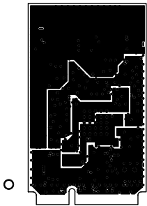
POWER PLANE LAYER 3 FULL RIVER (HK) LTD. WLB4E: 802.11a/b/g/n MINICARD REFERENCE DESIGN VER 1.0
