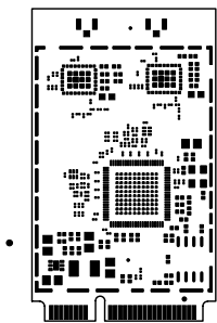
TOP SIDE SOLDERPASTE
