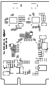
TOP SIDE SILKSCREEN FULL RIVER (HK) LTD. WLS4E: 802.11a/b/g/n MINICARD REFERENCE DESIGN VER 1.0
