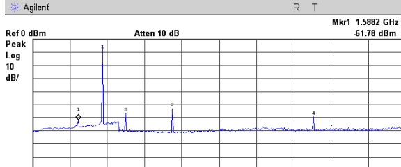
Figure 8. Plot of the Spurious RF conducted emissions
