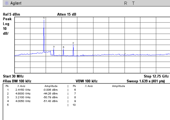
Figure 8. Plot of the Spurious RF conducted emissions
