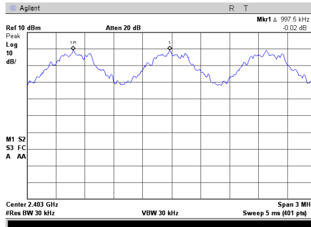
Figure 2. Plot of the Carrier Frequency Separation (Conducted)
