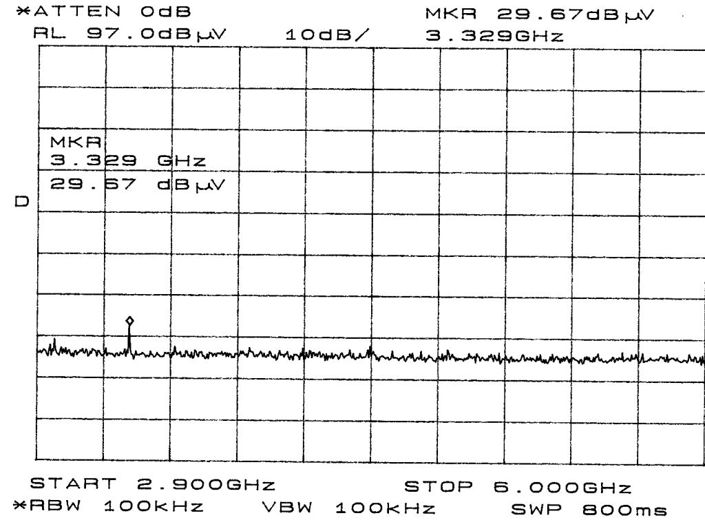
Figure four Plot of General Radiated Emissions
