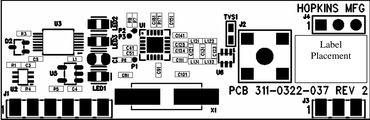
Top silk screen of PCB
