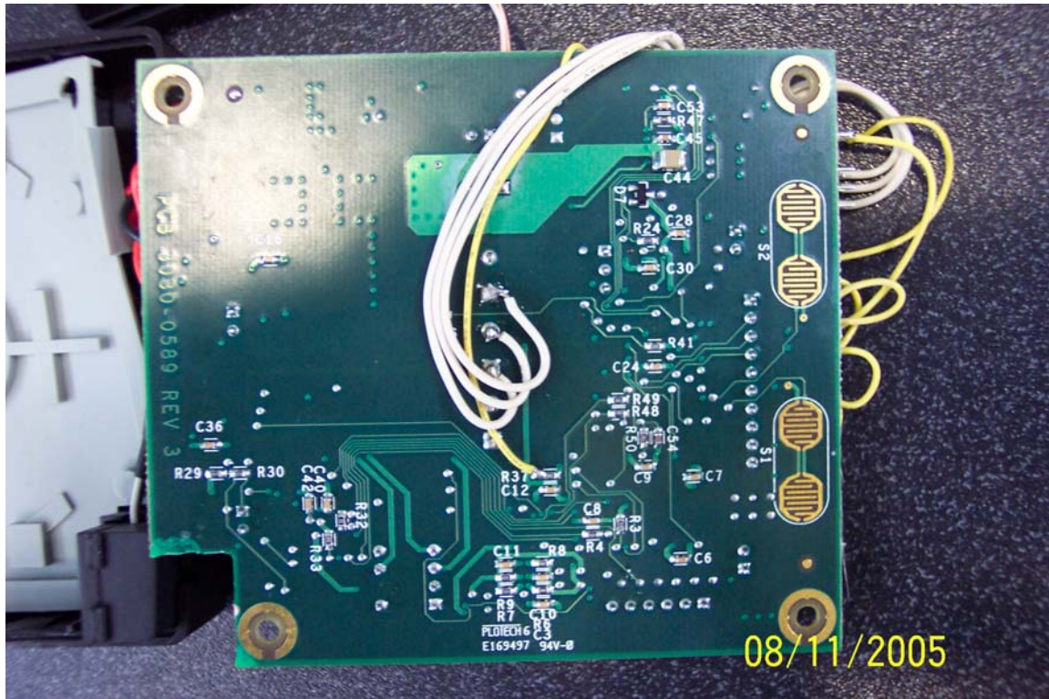
Internal Photograph 2 – Main PCB bottom view
