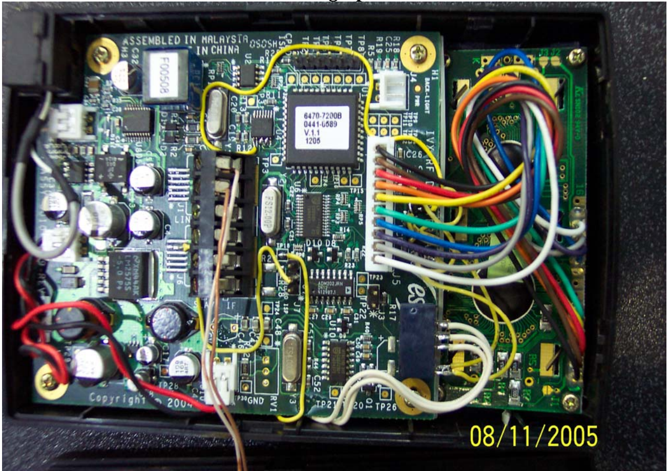
Internal Photograph 1 – Main PCB Top view
