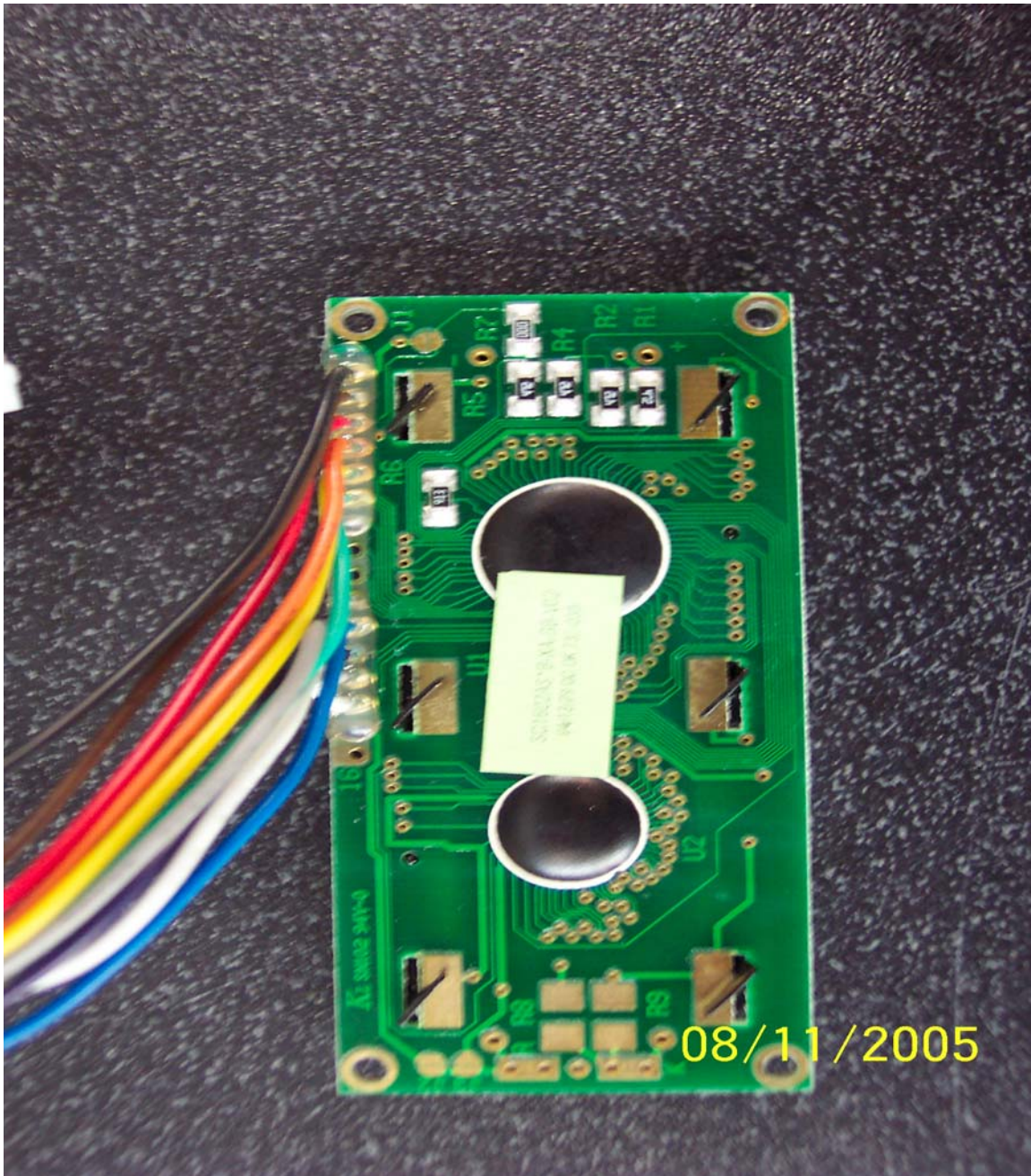
Internal Photograph 3 – LCD PCB bottom view
