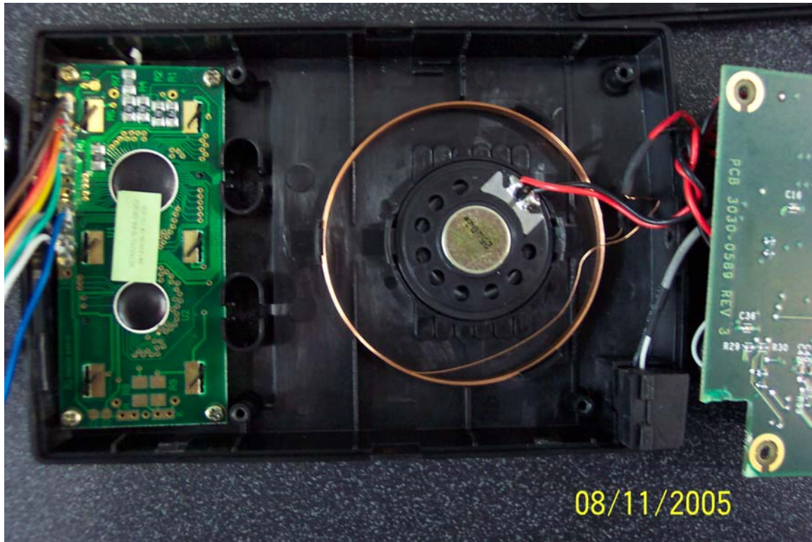
Internal Photograph 5 – Inside view showing antenna
