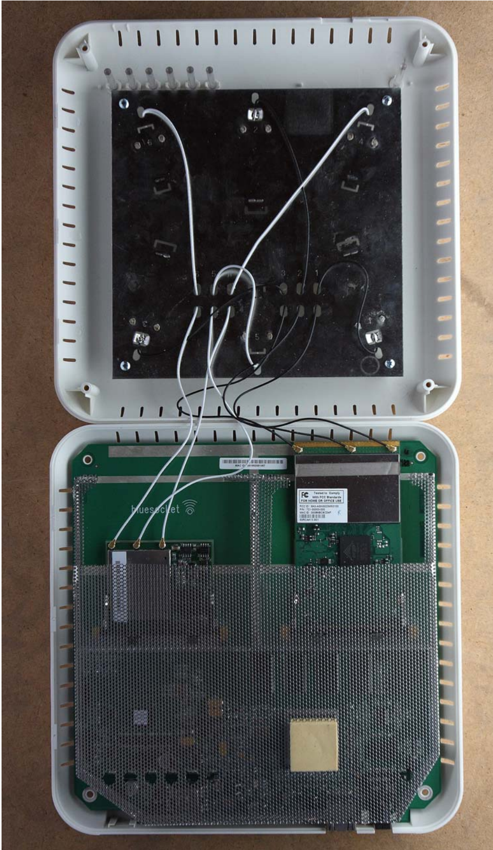
Main Board in Case - Front
