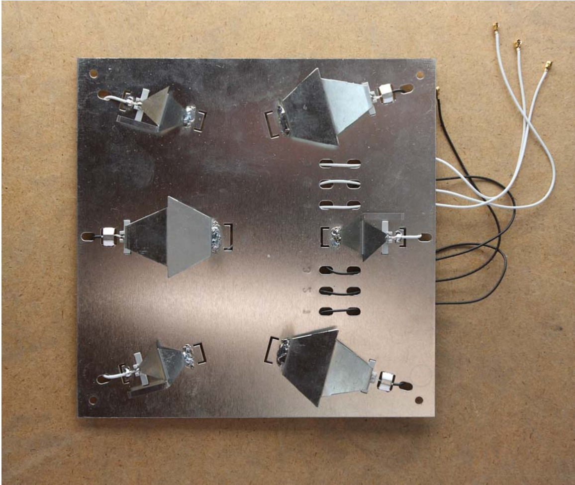
Internal Photos - BSAP-1800 Antenna - Bottom Side
