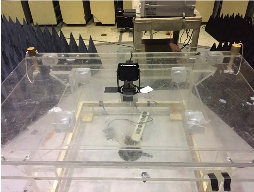
Radiated Emissions to 26.5 GHz, Front
