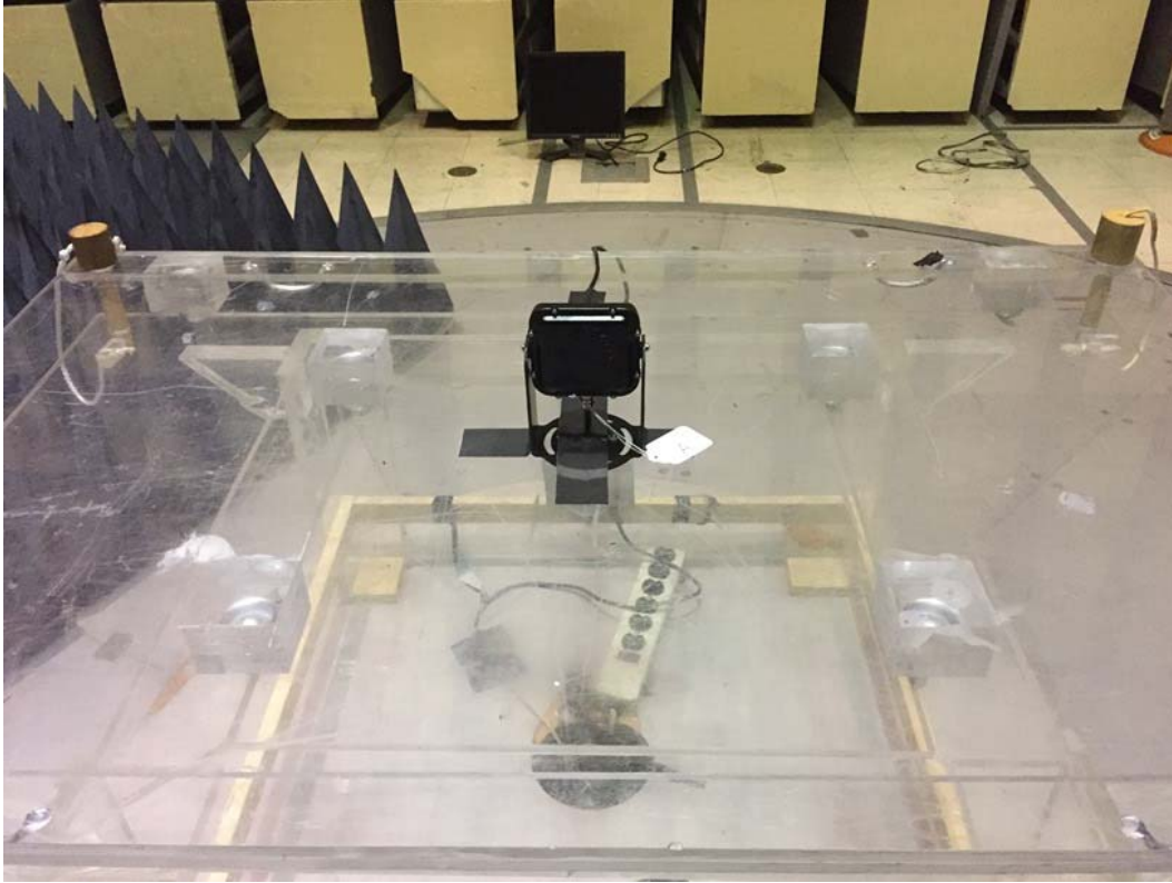
Radiated Emissions to 18 GHz, Front
