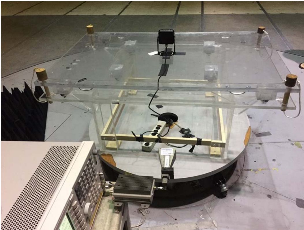
Radiated Emissions to 26.5 GHz, Back
