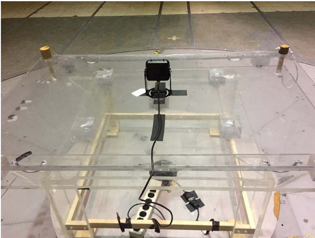
Radiated Emissions to 18 GHz, Back
