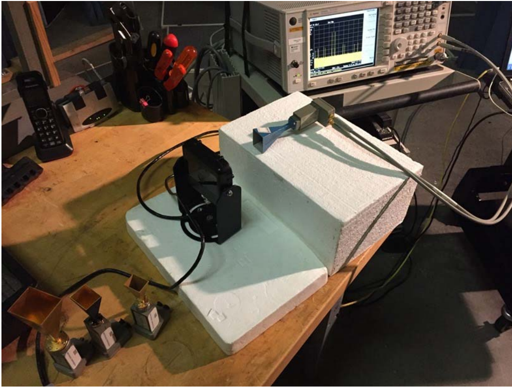
Radiated Emissions to 100 GHz
