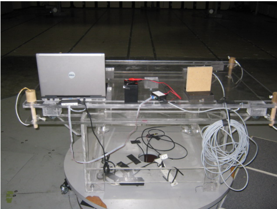
Radiated Emissions Below 1 GHz – Back View
