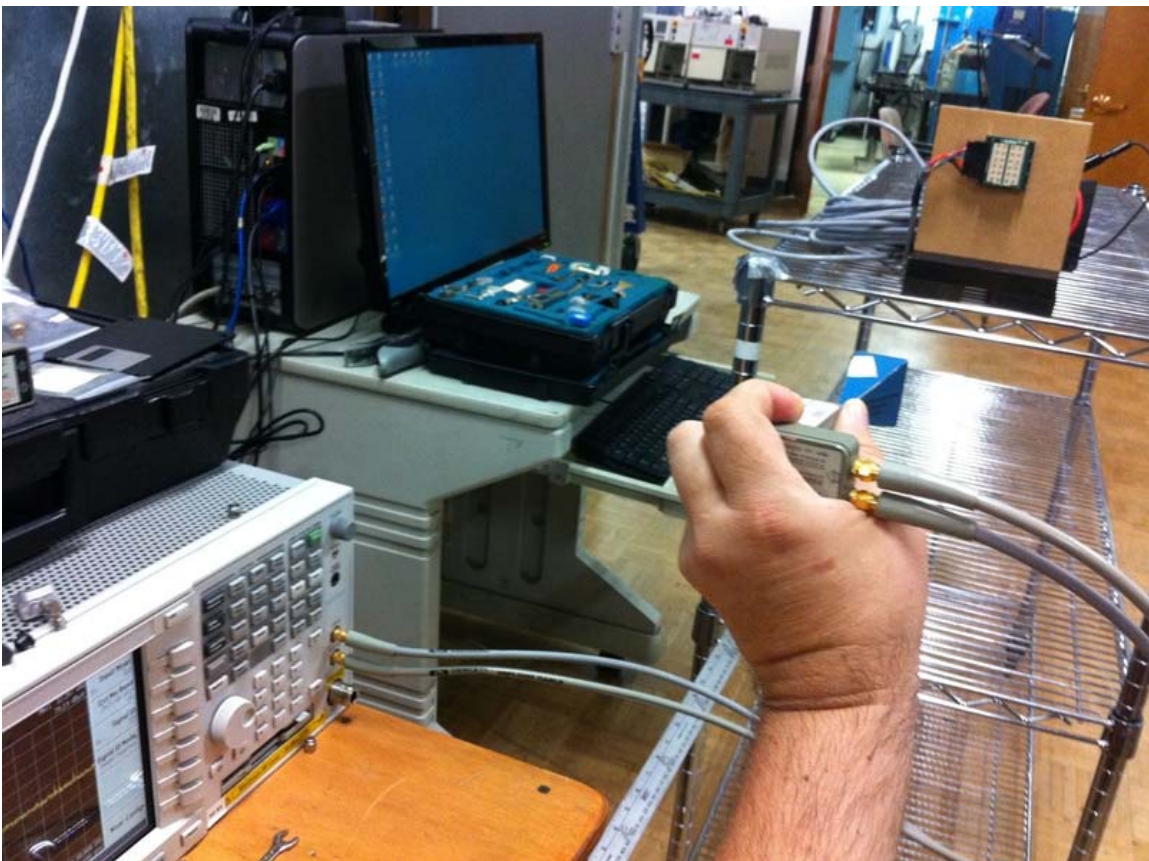
Radiated Emissions 30 GHz to 100 GHz
