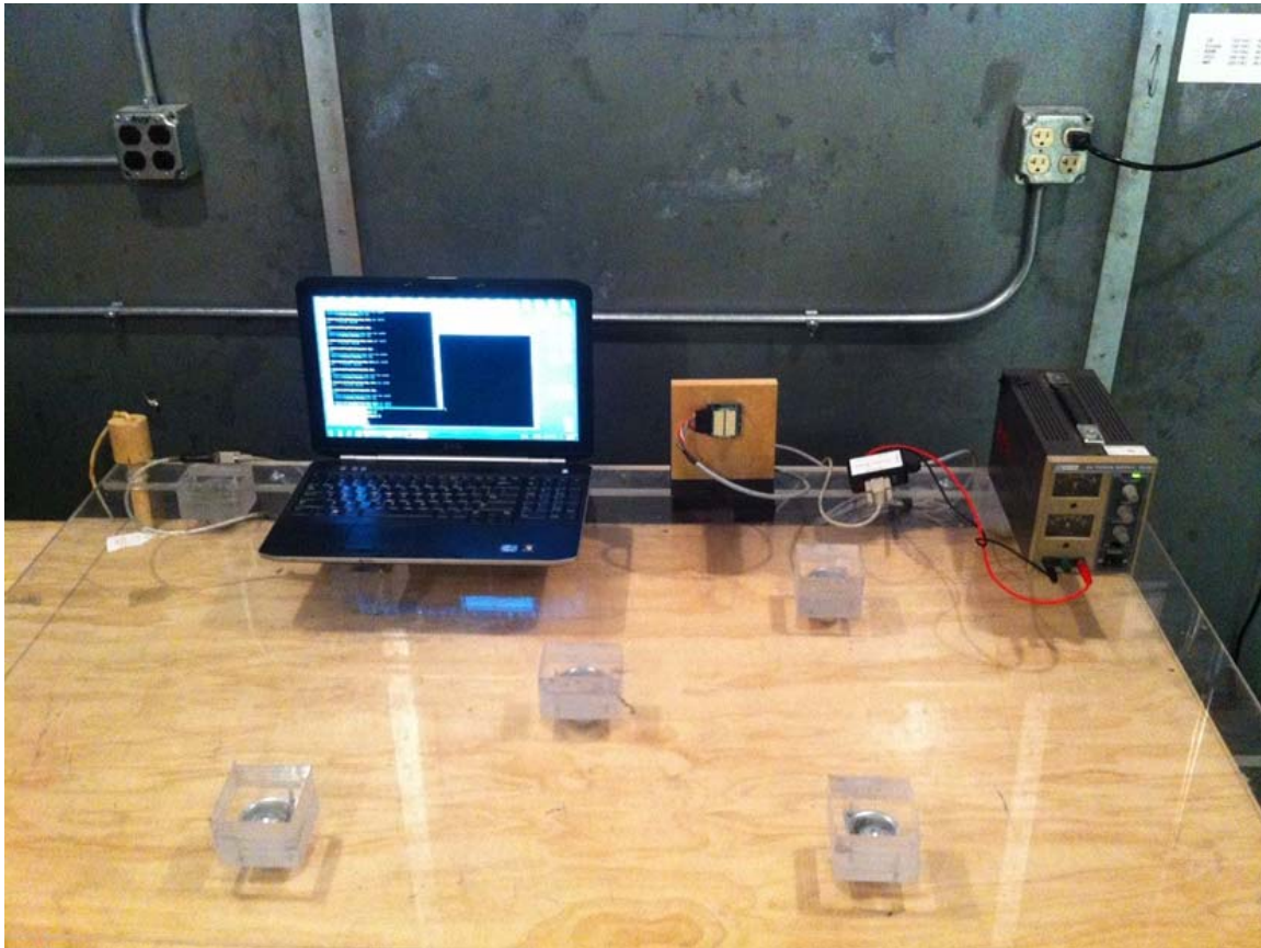
AC Mains Conducted Emissions, 1 of 3
