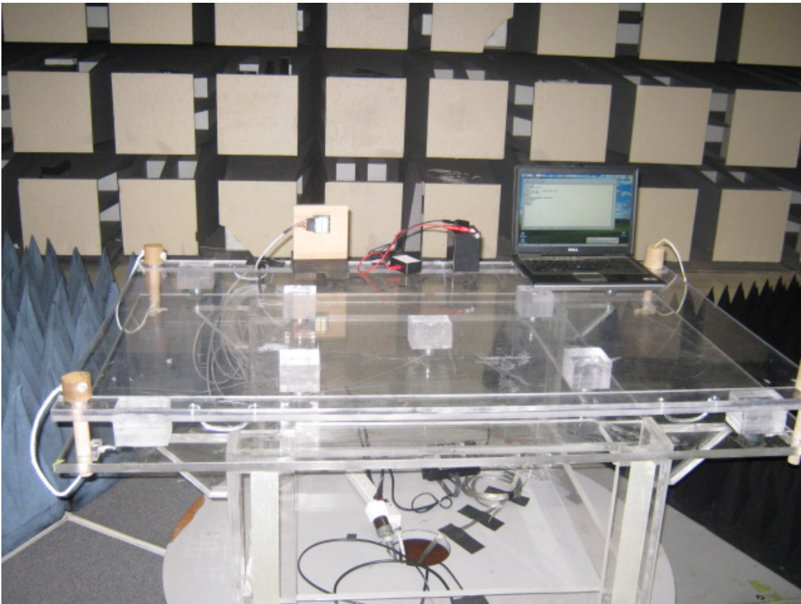
Radiated Emissions Below 1 GHz – Front View
