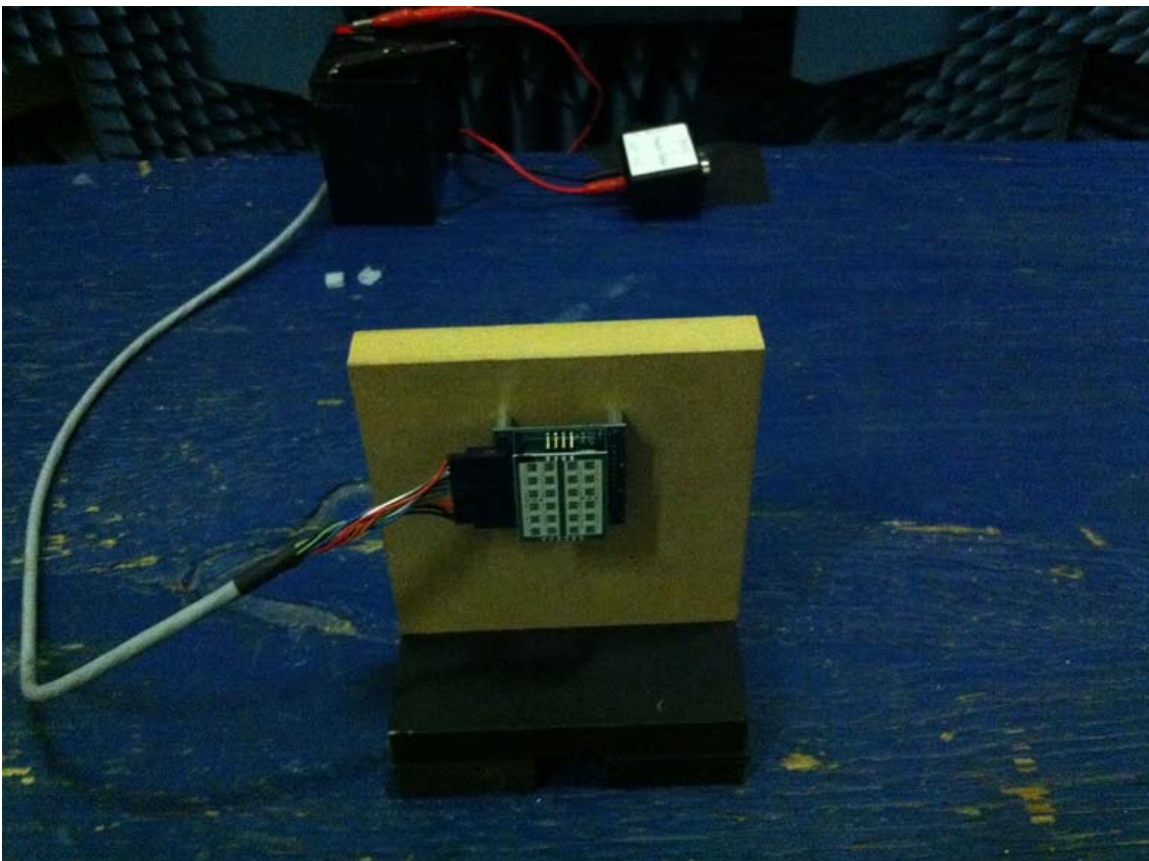
Radiated Emissions 1 GHz to 30 GHz – Close View
