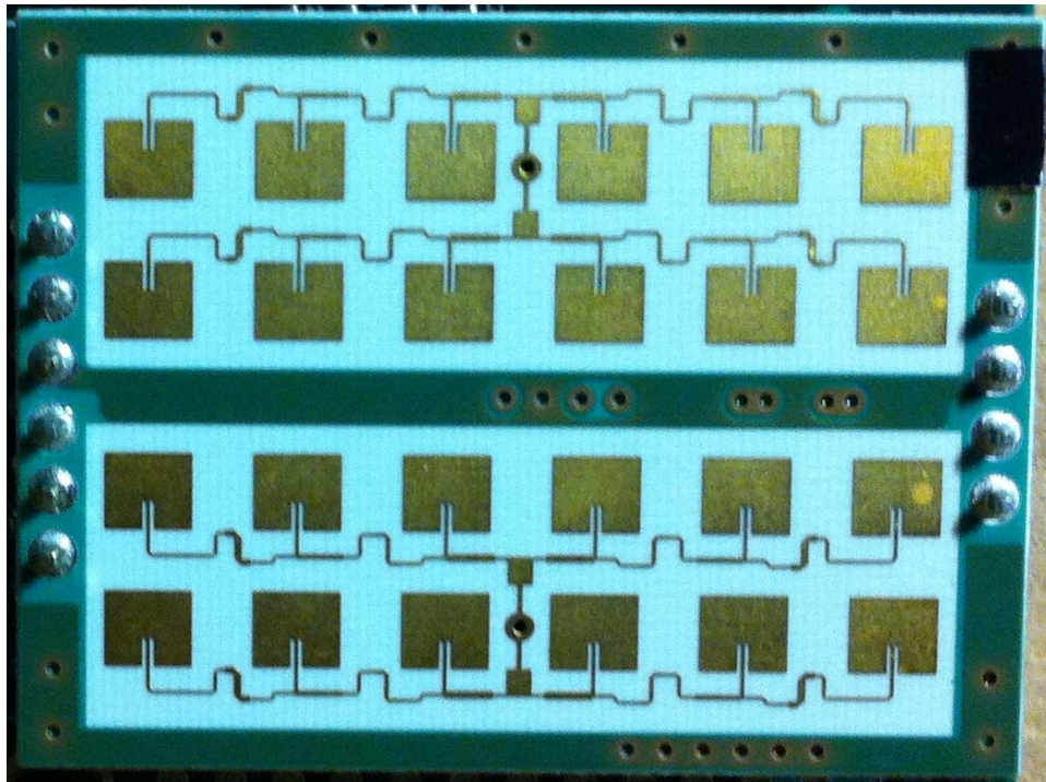
IPS-223 RF Section - Bottom Side View – Antenna - This surface is not coated.
