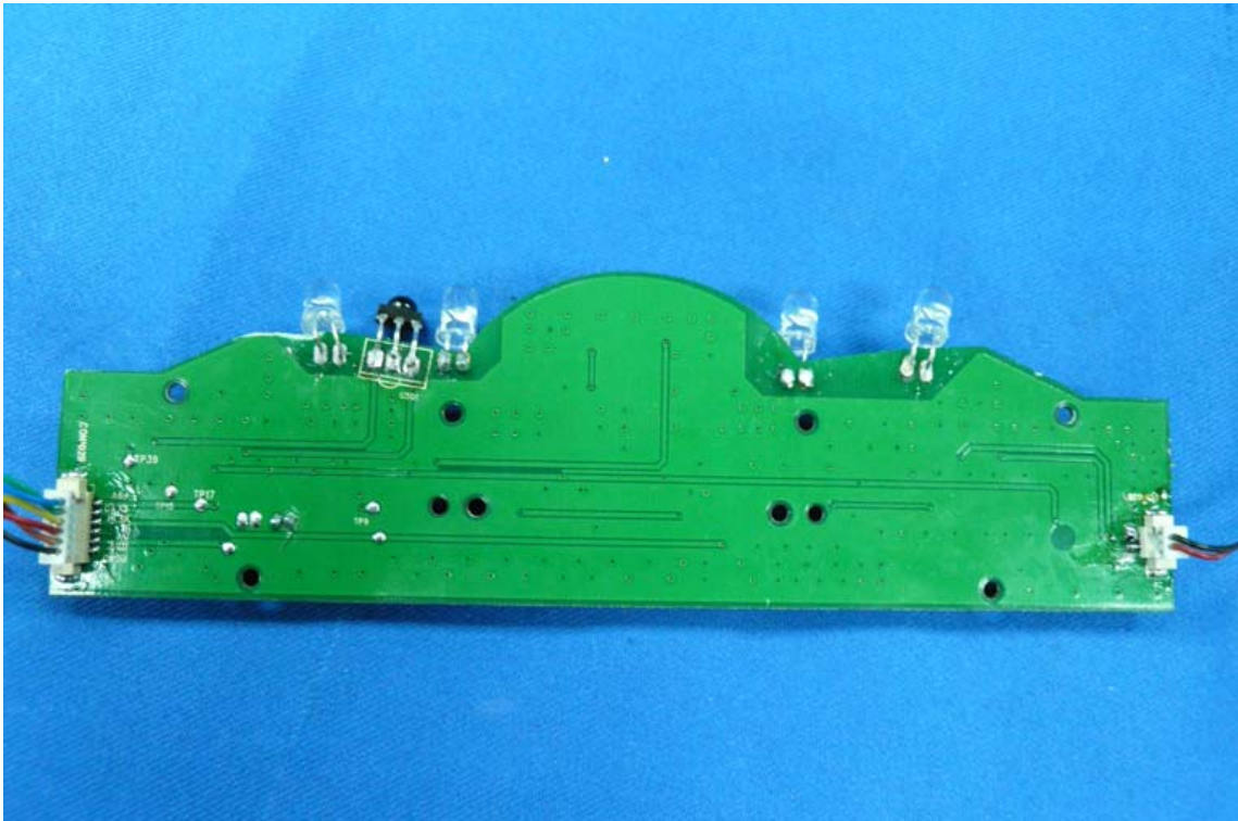
Figure 16 Control board of the EUT
