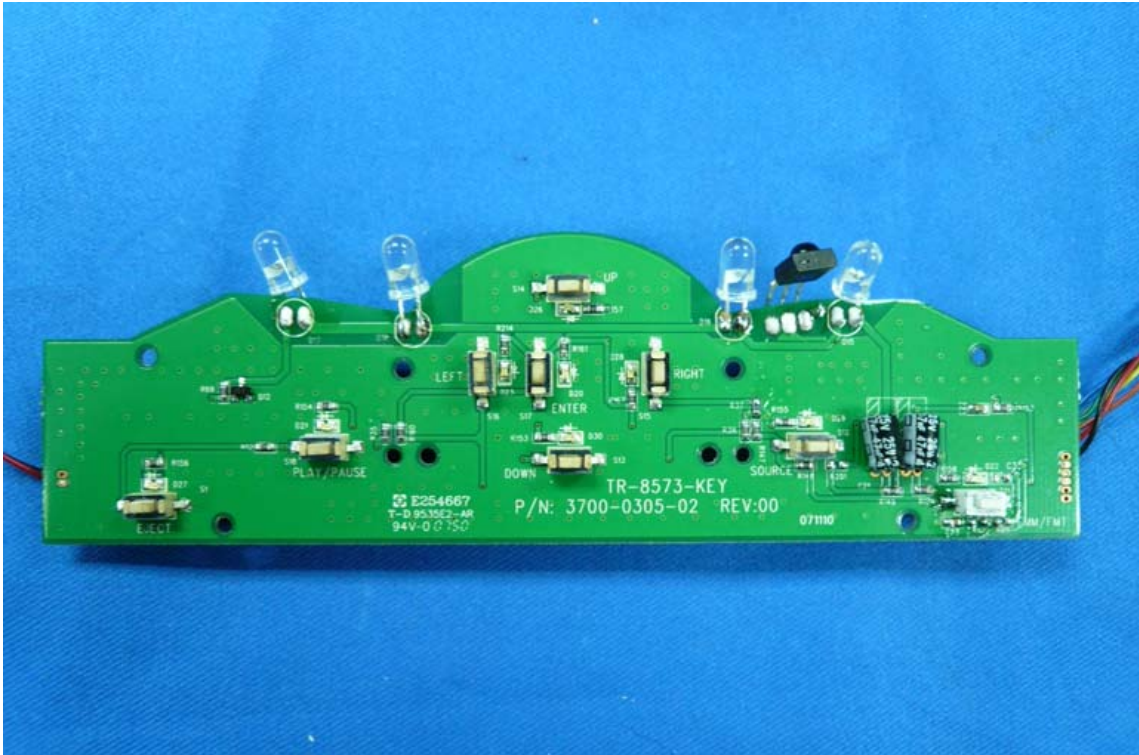
Figure 15 Control board of the EUT
