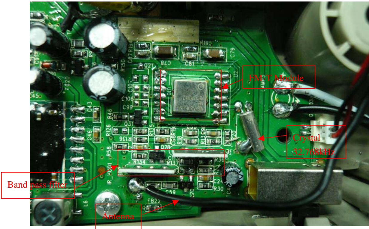
Figure 21 Inside of the EUT
