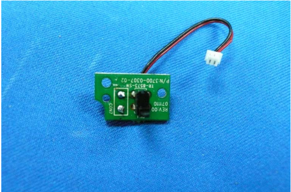
Figure 13 Inside of the EUT
