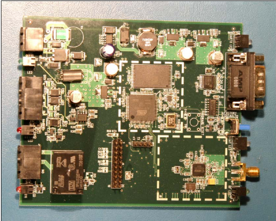
Photograph 2. LRT Internal Photo PCB Top View
