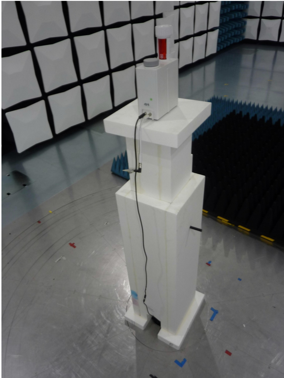
Test setup semi anechoic chamber (above 1 GHz)
