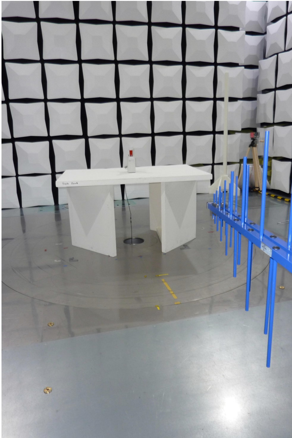
Test setup semi anechoic chamber (30 MHz to 1 GHz)
