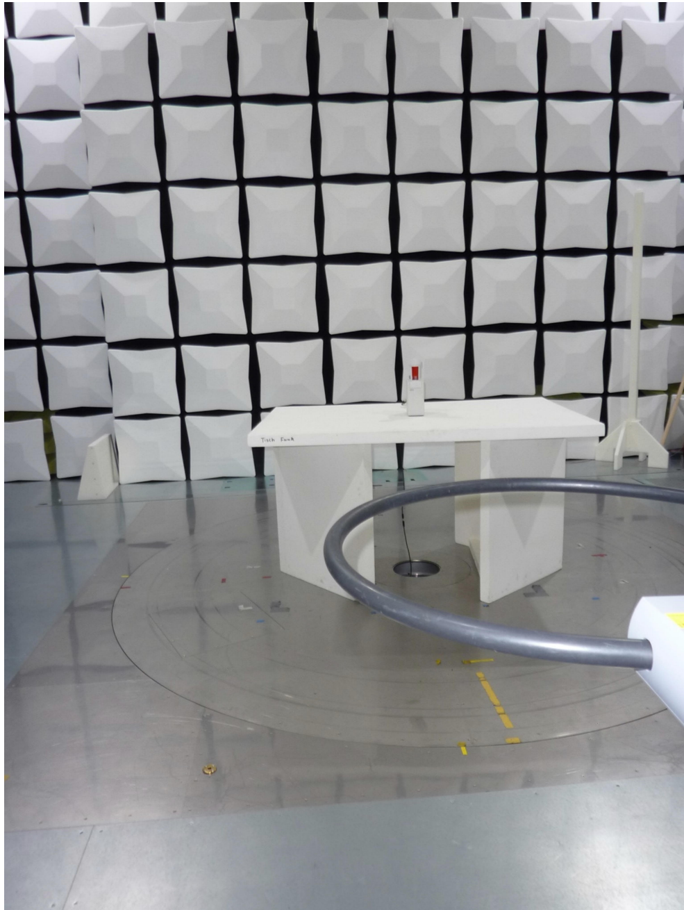
Test setup semi anechoic chamber (150 kHz to 30 MHz)
