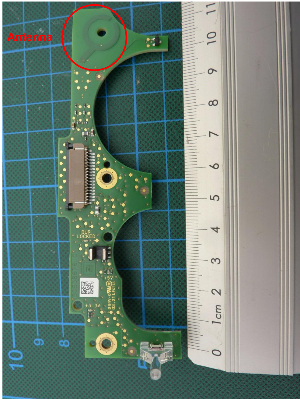
DoserDetectionRFID PCB, top view
