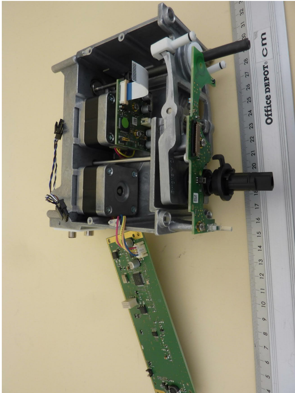
Internal view 3 (view to PCBs)
