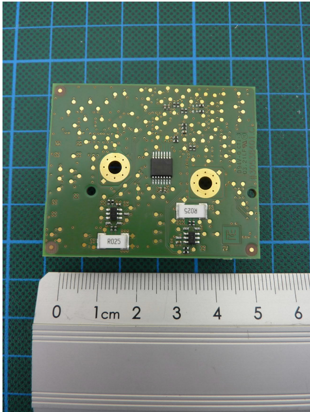
MotorControlFOC PCB, bottom view
