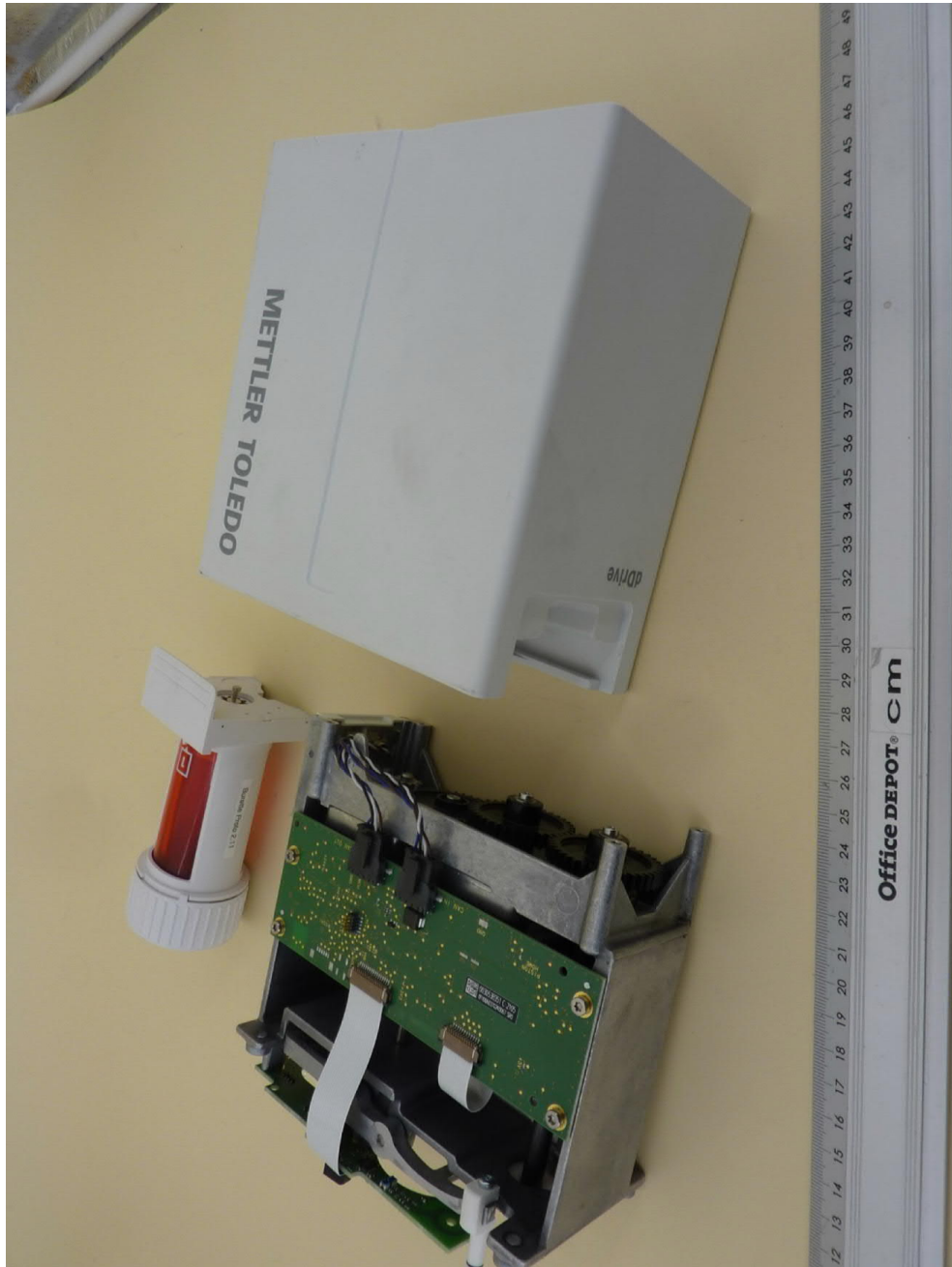
Internal view 2 (housing removed)
