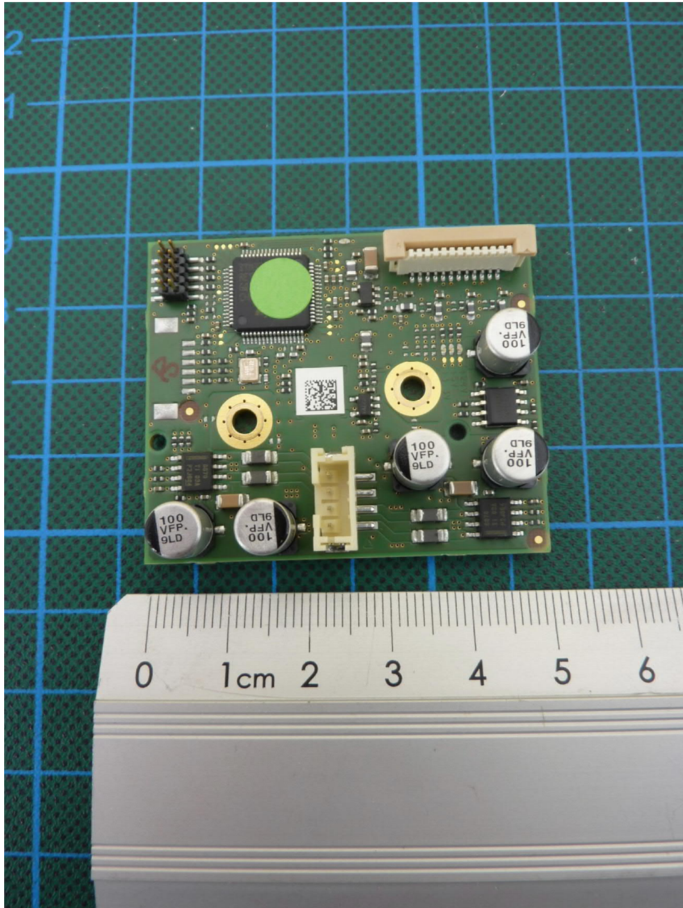
MotorControlFOC PCB, top view
