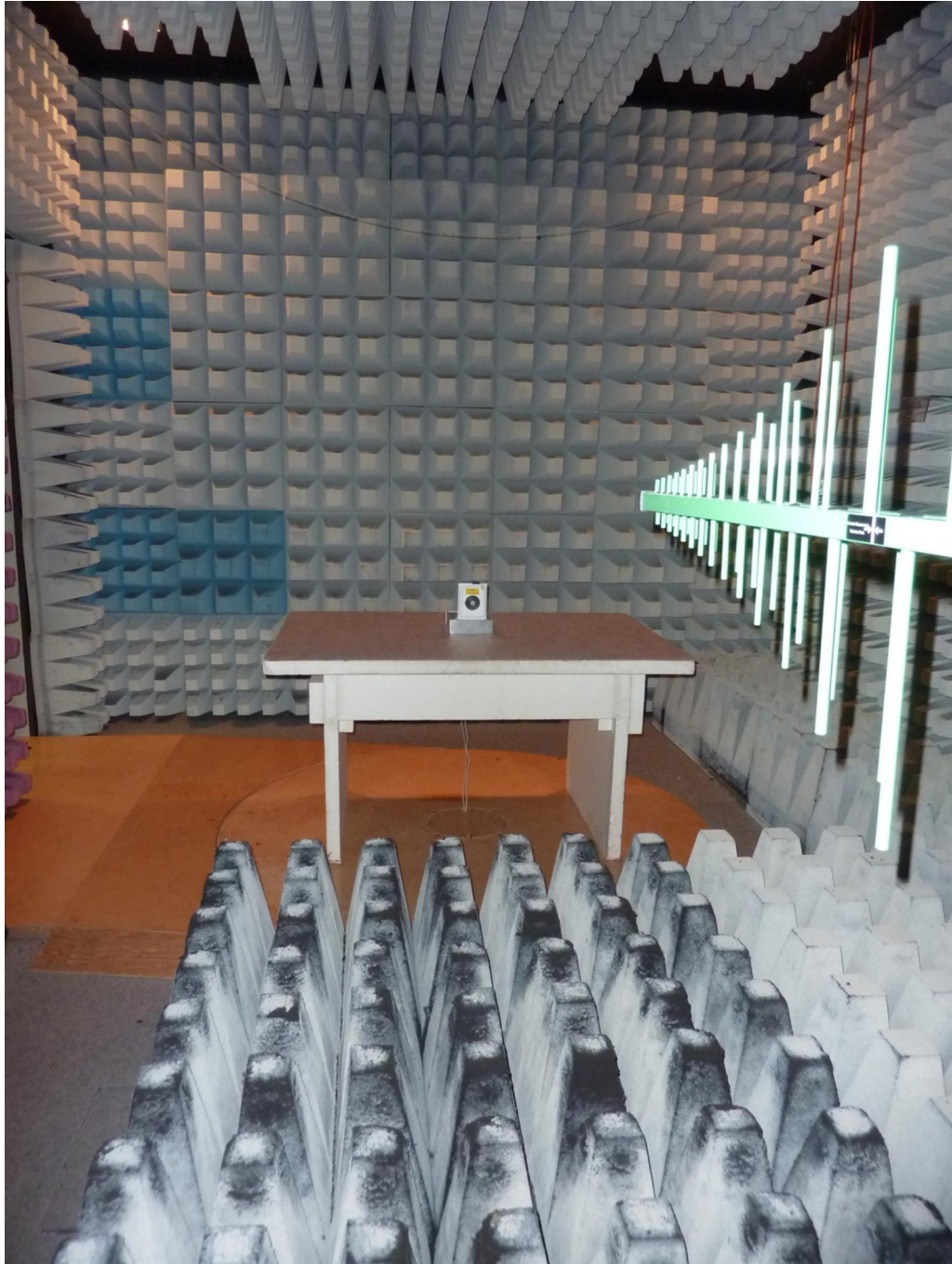
172416_9.jpg: SmartScan, test set-up fully anechoic chamber
