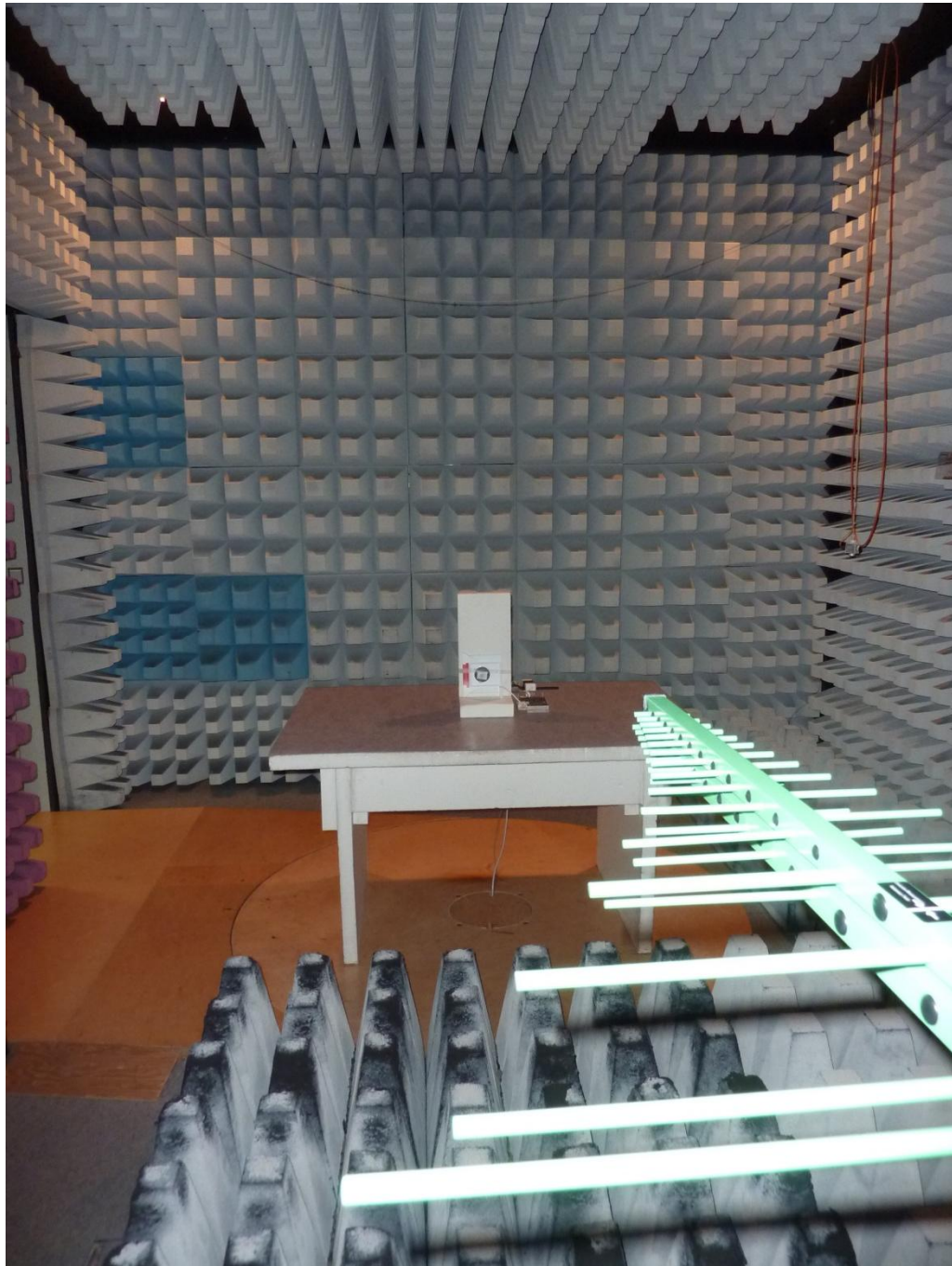
161000_i.jpg: SmartSample, test setup fully anechoic chamber
