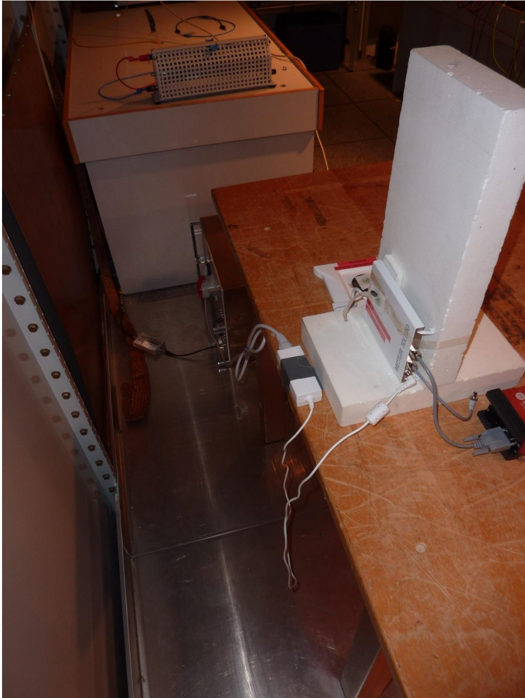
161000_I.jpg: SmartSample, test setup shielded chamber
