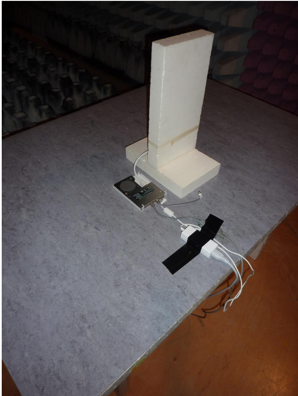
161000_k.jpg: SmartSample, test setup fully anechoic chamber
