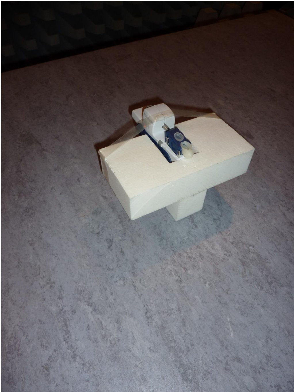
161007_1a.jpg: Quantos HPD, test setup fully anechoic chamber, Position 2
