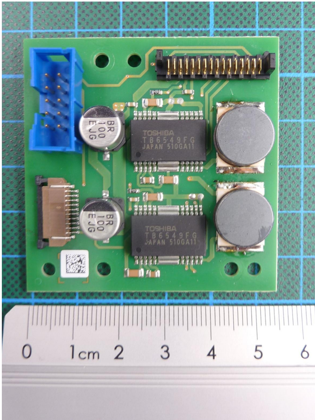
161005_18.jpg: Q2 powder dosing unit, PCB 3, top view
