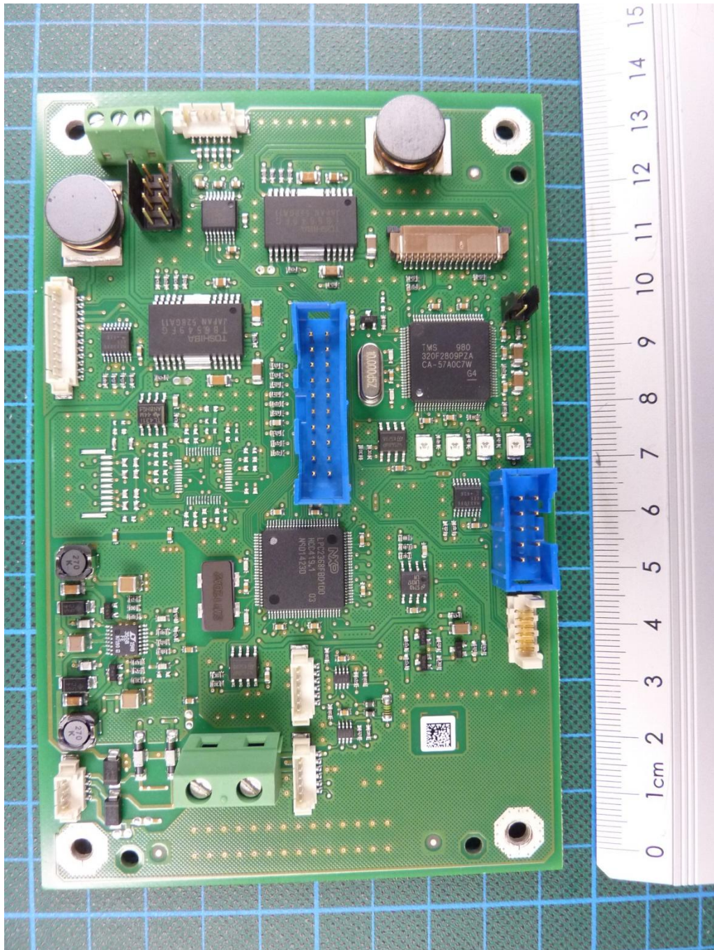
161005_14.jpg: Q2 powder dosing unit, PCB 1, top view
