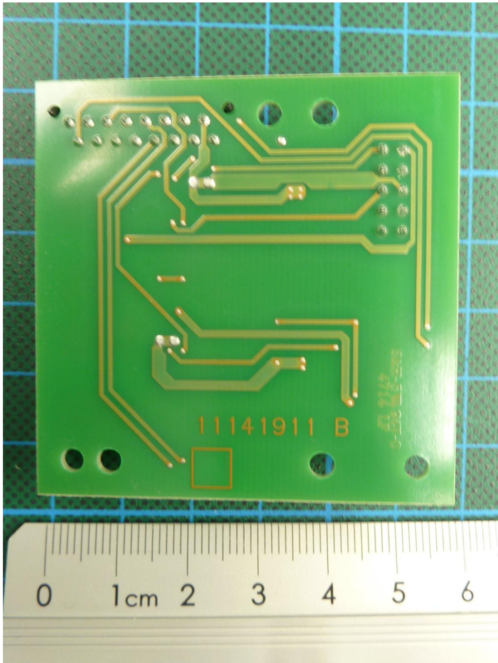
161005_19.jpg: Q2 powder dosing unit, PCB 3, bottom view
