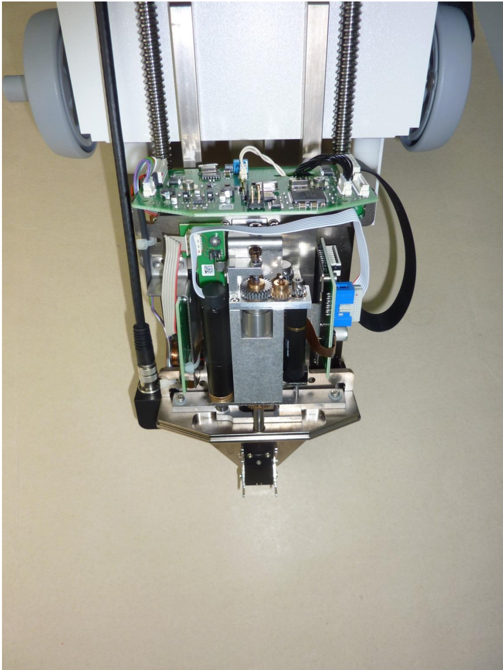
161005_11.jpg: Q2 powder dosing unit, internal view, front cover removed
