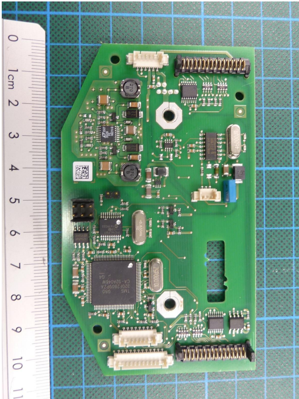
161005_16.jpg: Q2 powder dosing unit, PCB 2, top view
