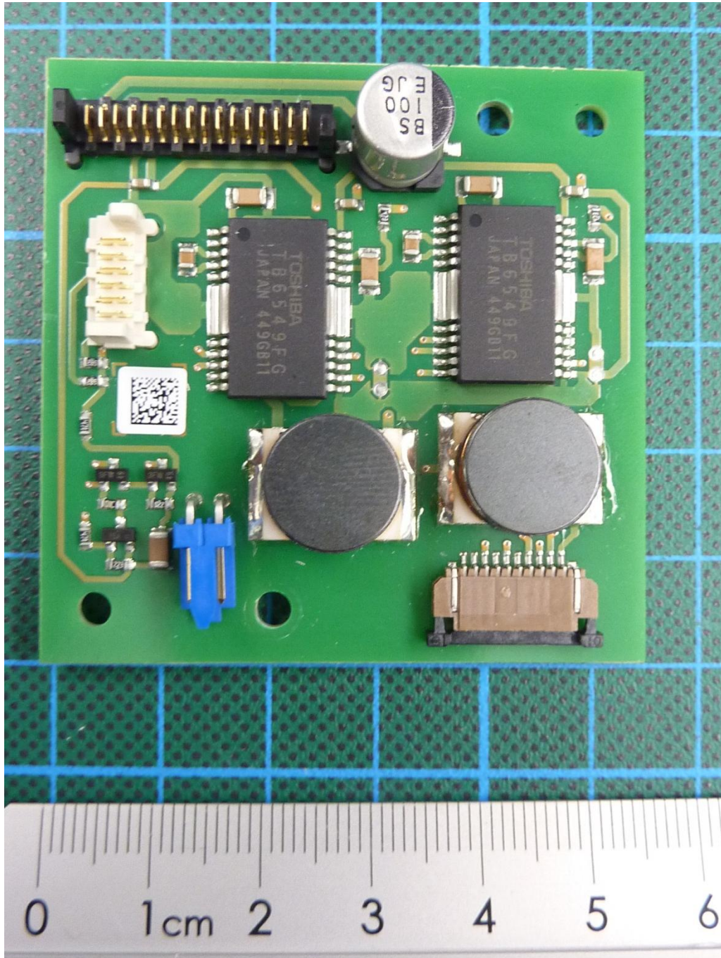
161005_20.jpg: Q2 powder dosing unit, PCB 4, top view
