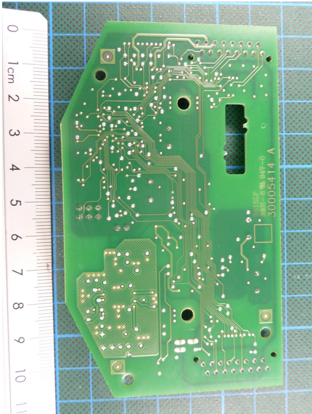
161005_17.jpg: Q2 powder dosing unit, PCB 2, bottom view
