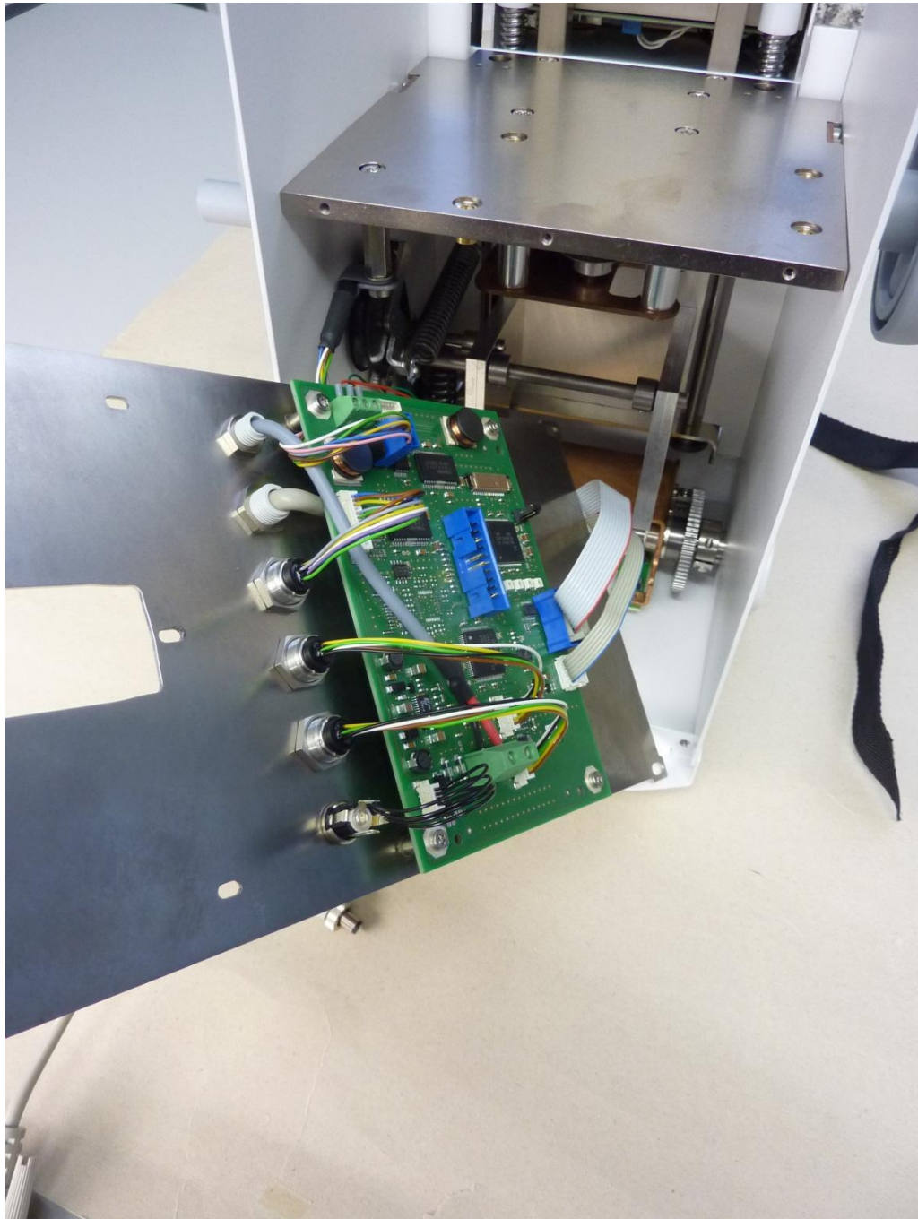
161005_12.jpg: Q2 powder dosing unit, internal view, rear cover removed
