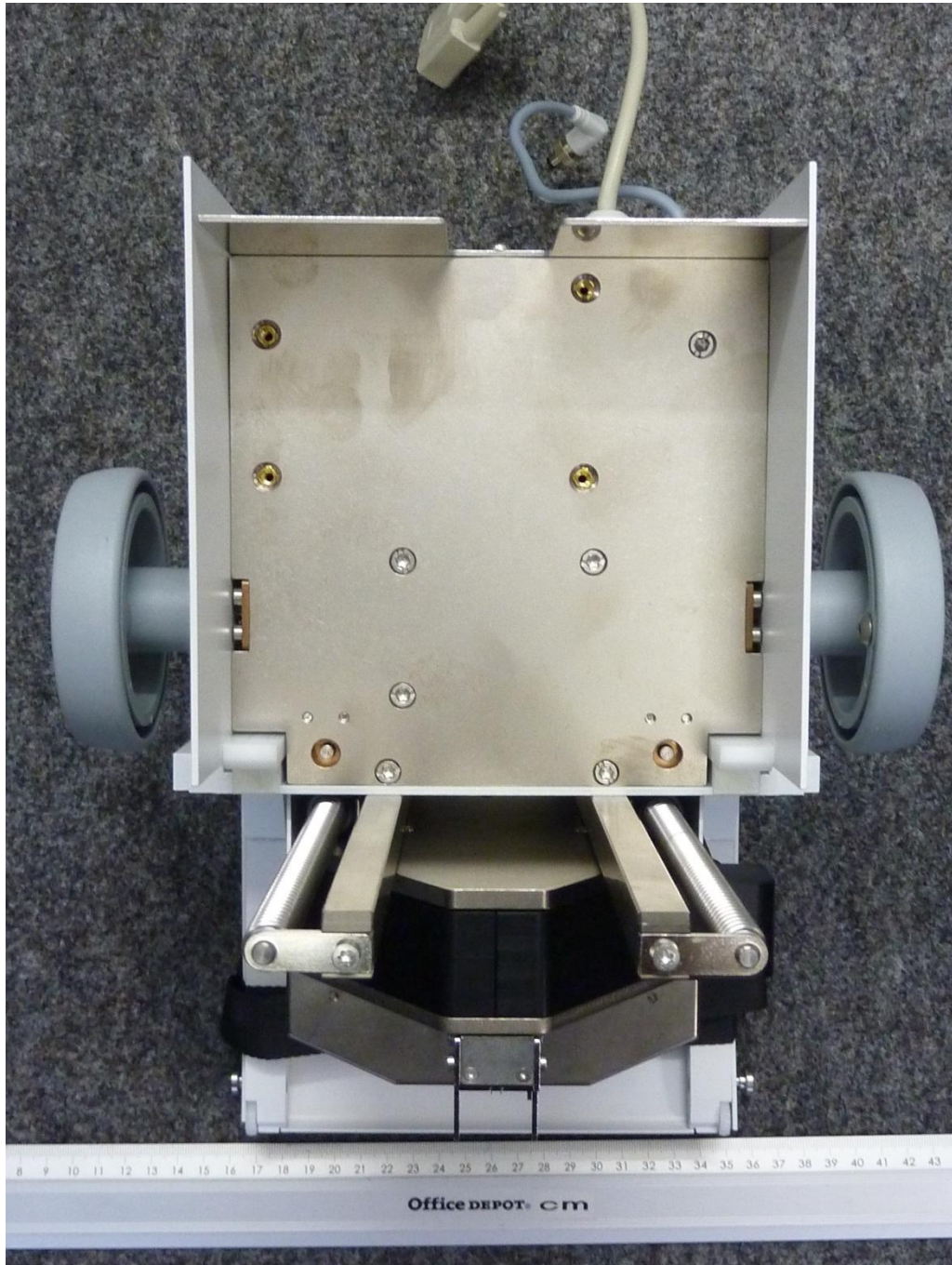
161005_5.jpg: Q2 powder dosing unit, bottom view
