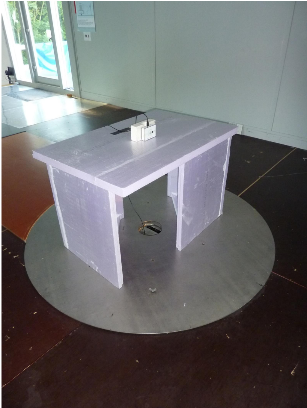
172414_12.jpg: EasyScan USB, test set-up open area test site
