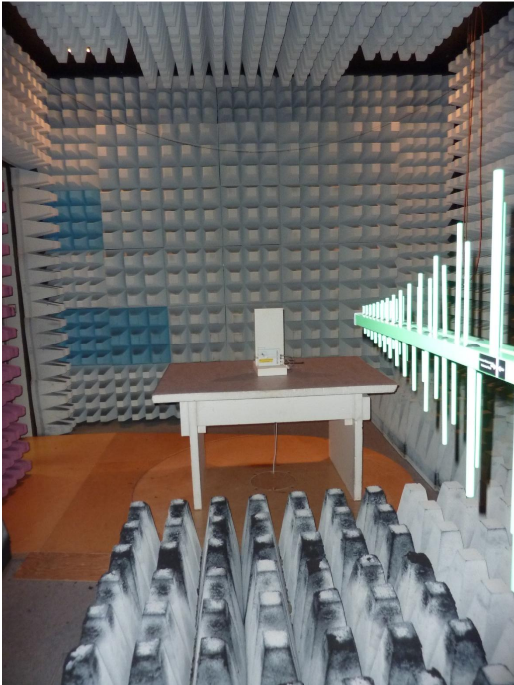
160874_k.jpg: EasyScan Module, test setup fully anechoic chamber
