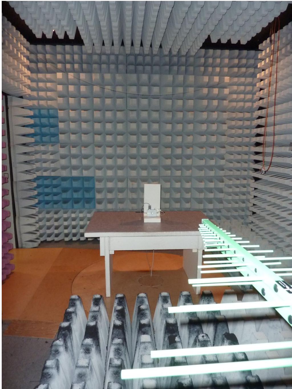
161004_k.jpg: EasyScan Flex, test setup fully anechoic chamber
