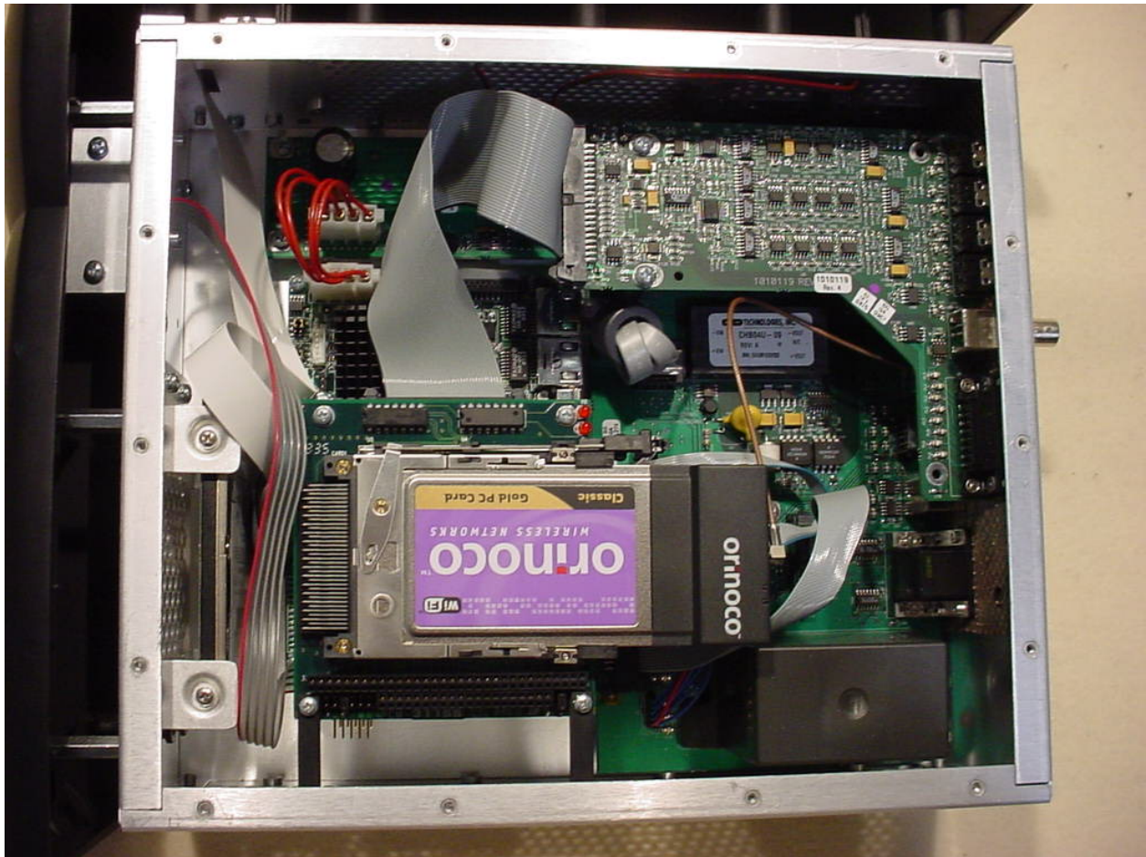
Figure C.1 – System View
