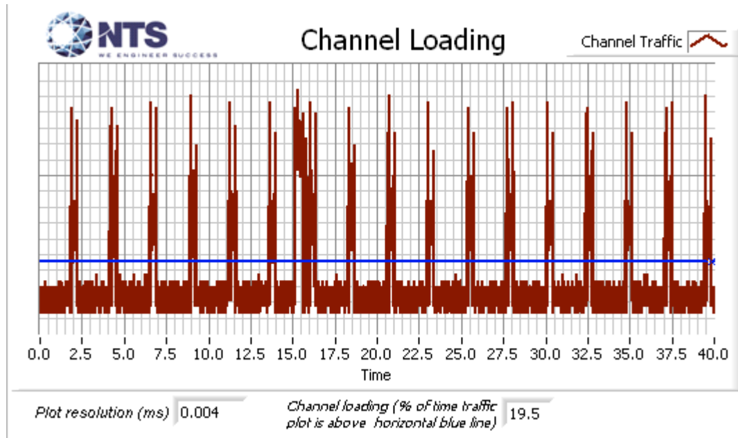
Figure 12 - Channel Loading
