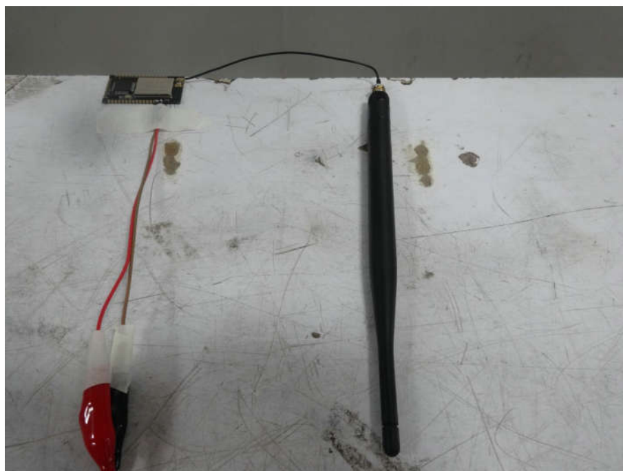
Conducted Emissions Test Setup for close-up
