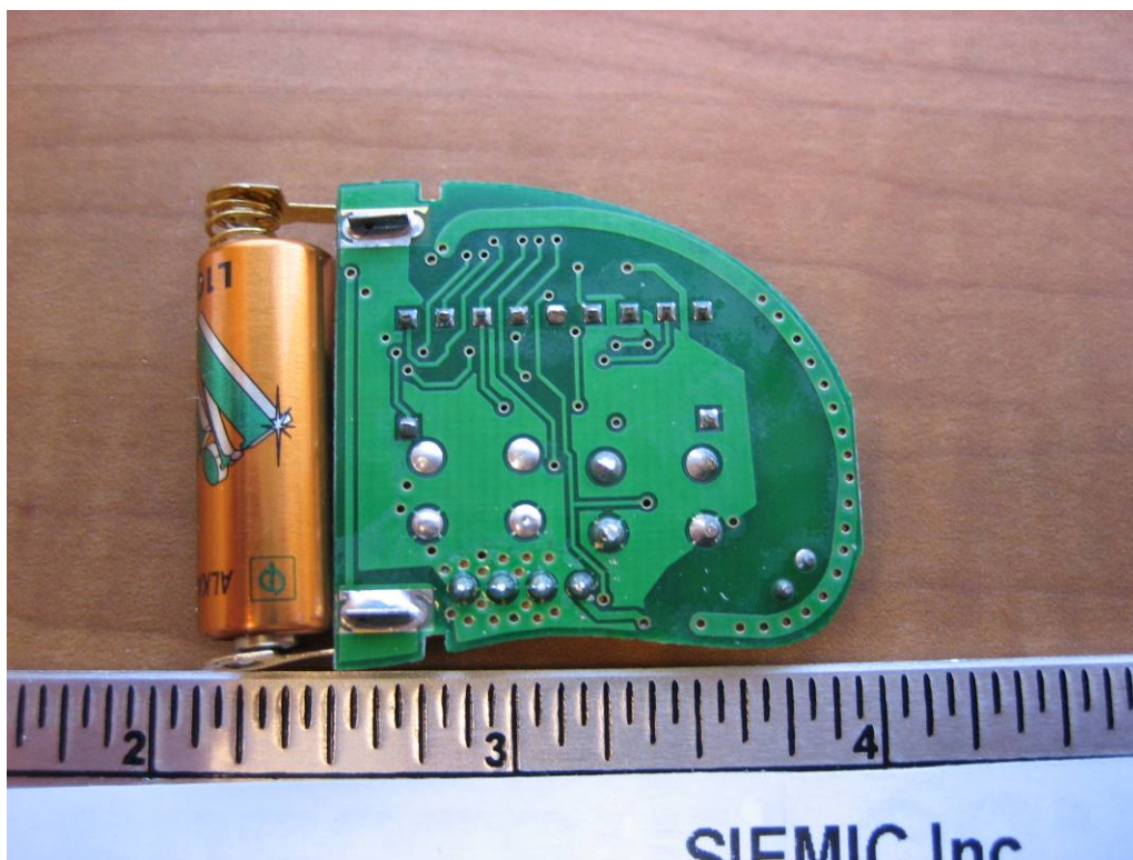
Board Bottom View
