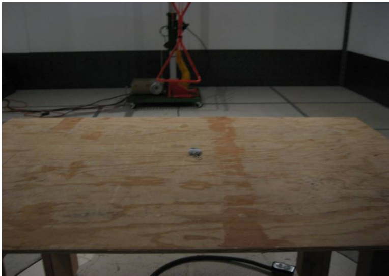
Radiated Emission Test Setup Rear View
